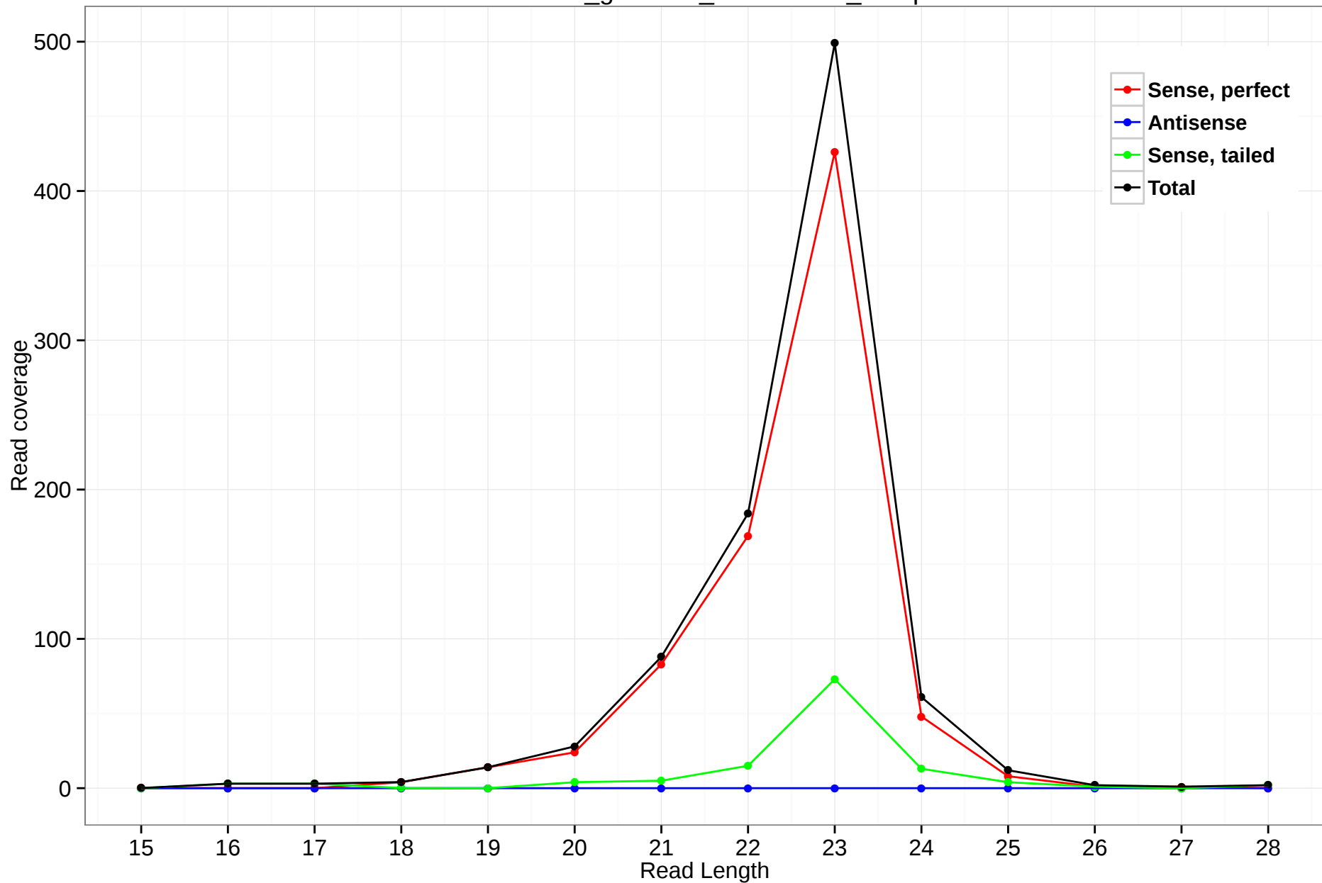
rheMac3_genscan_chr11.1015_35.3p
