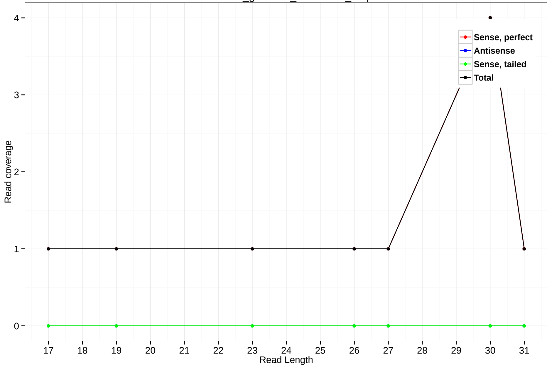
rheMac3_genscan_chr10.917_7.3p
