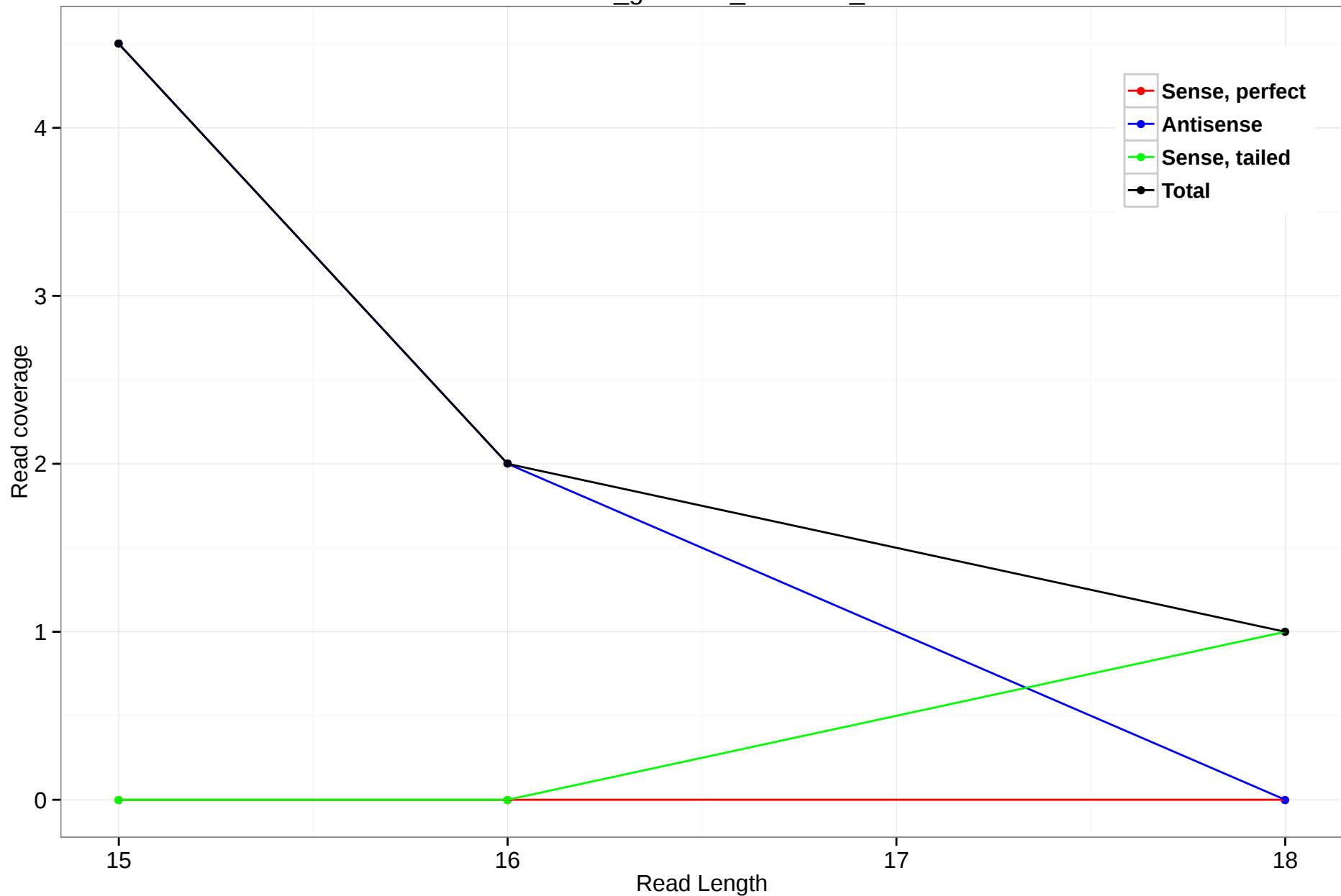
rheMac3_genscan_chr10.90_69
