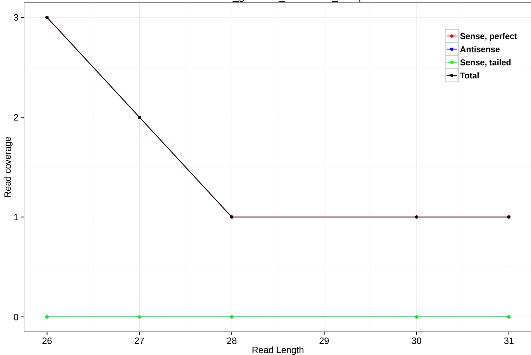
rheMac3_genscan_chr10.878_15.3p
