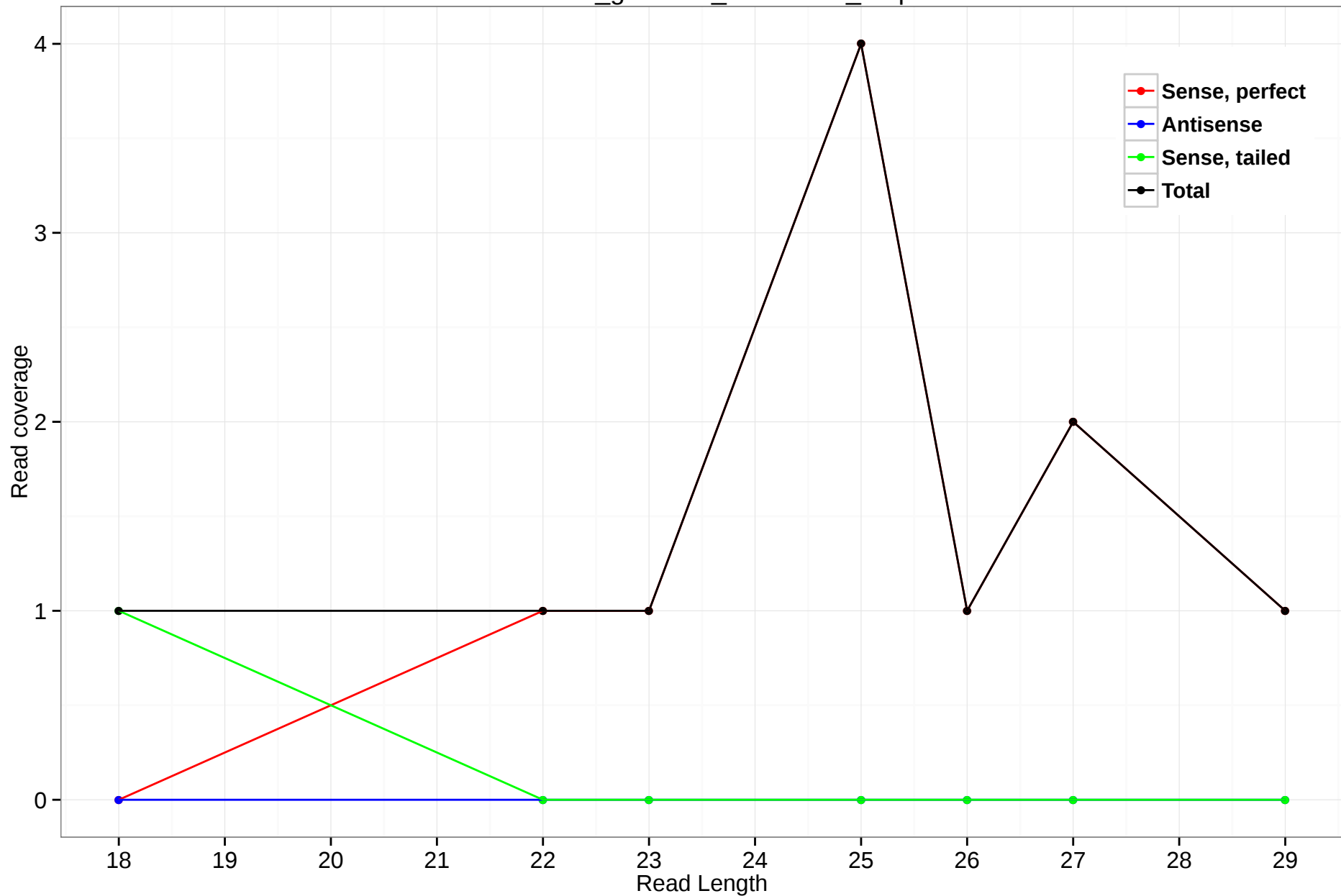
rheMac3_genscan_chr10.873_0.5p
