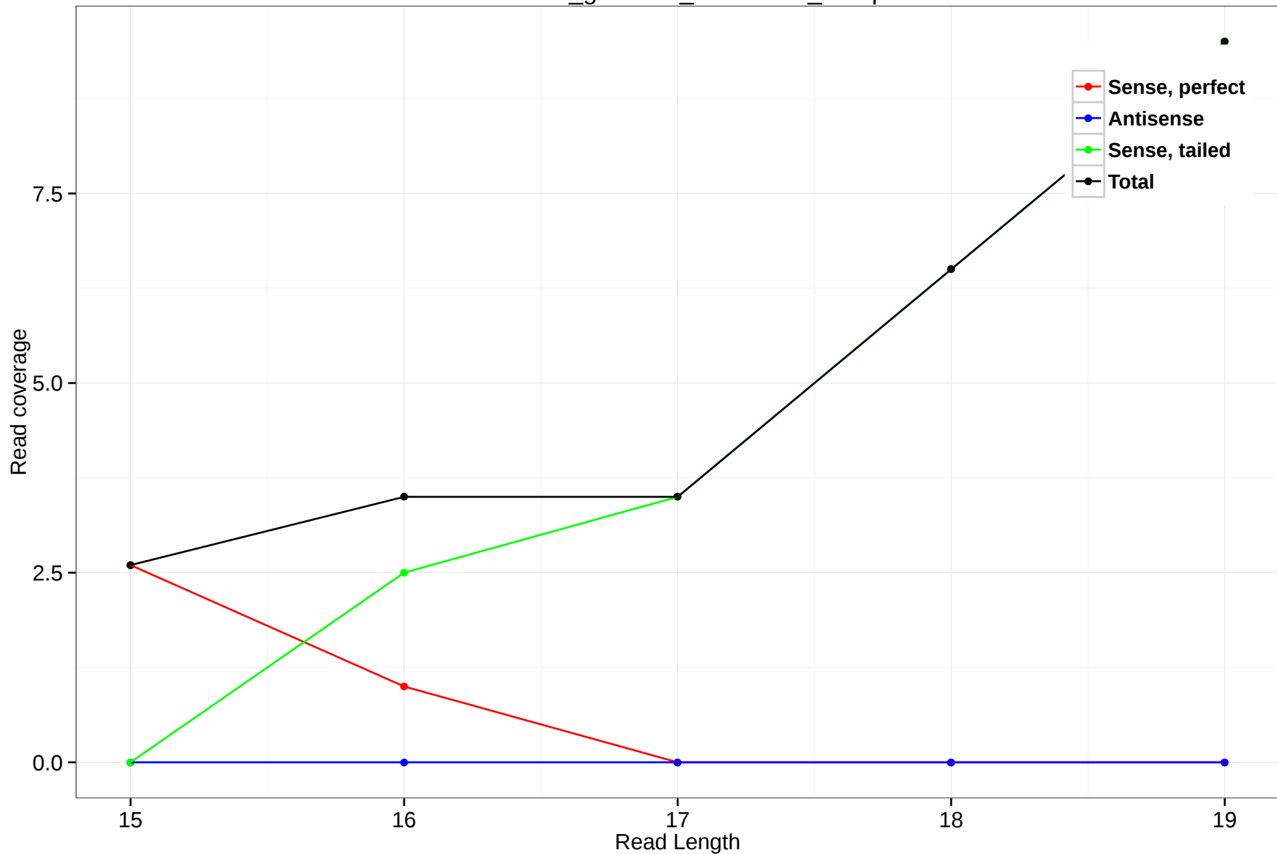
rheMac3_genscan_chr10.843_10.5p
