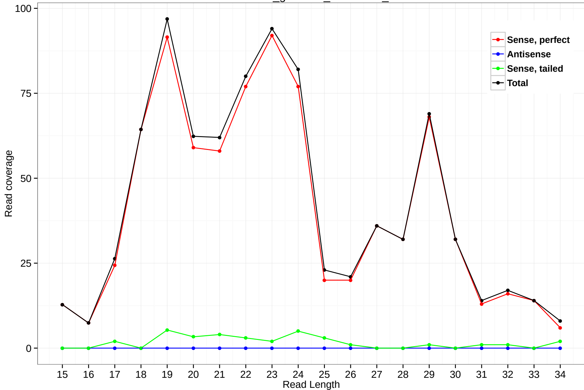
rheMac3_genscan_chr10.841_4
