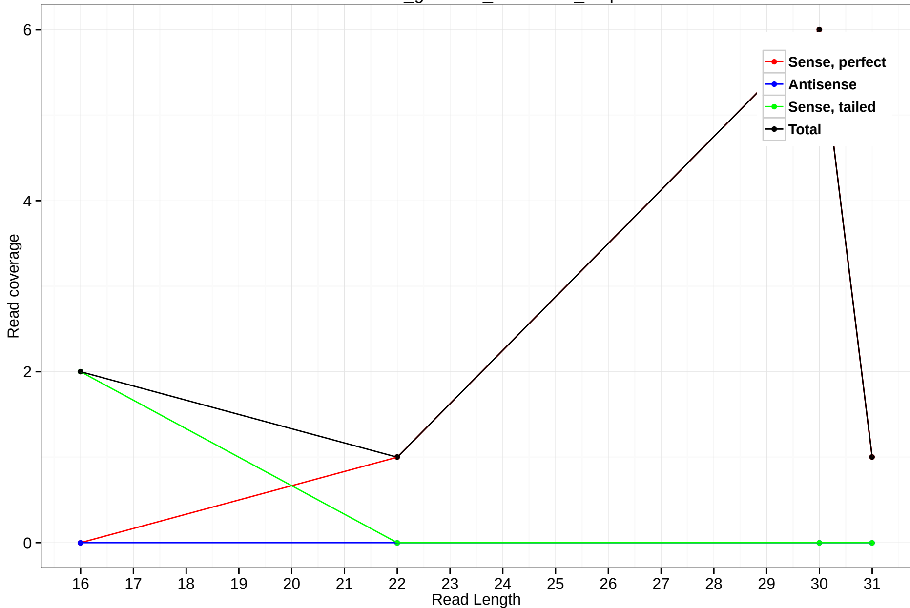
rheMac3_genscan_chr10.806_9.3p
