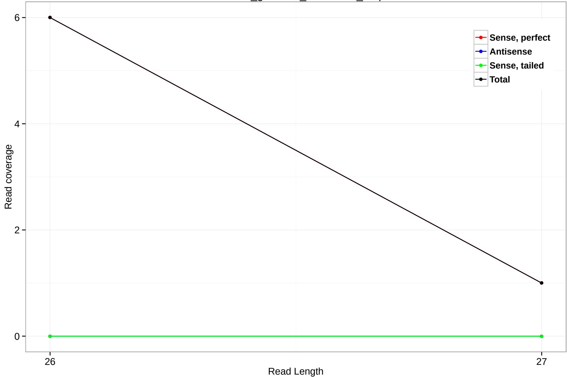
rheMac3_genscan_chr10.782_5.3p
