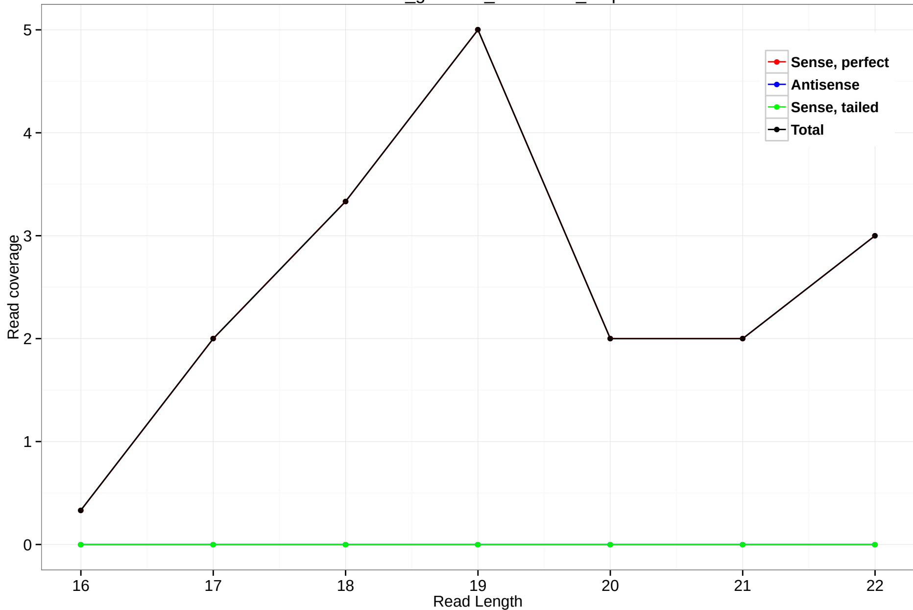
rheMac3_genscan_chr10.781_1.5p
