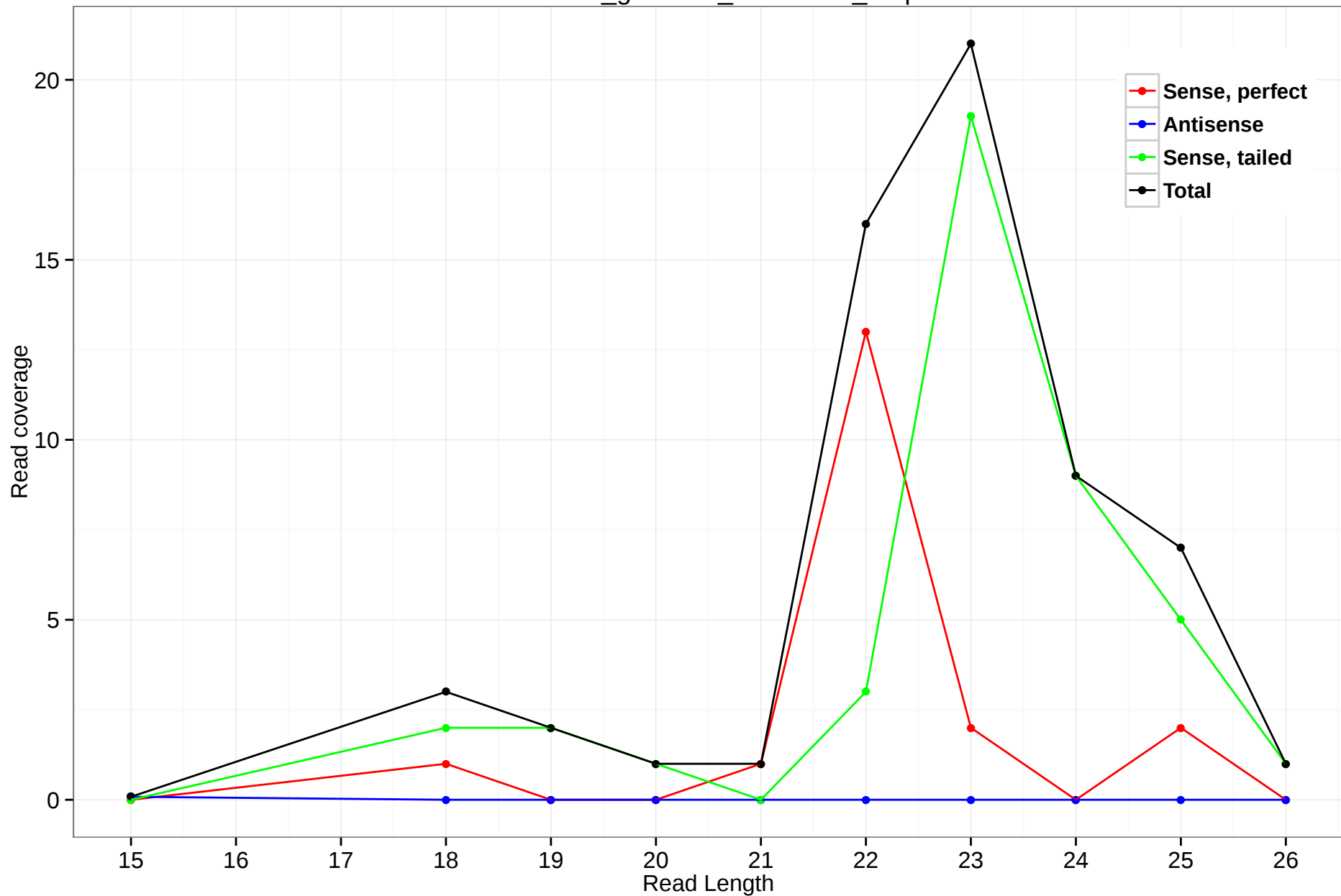
rheMac3_genscan_chr10.767_6.3p
