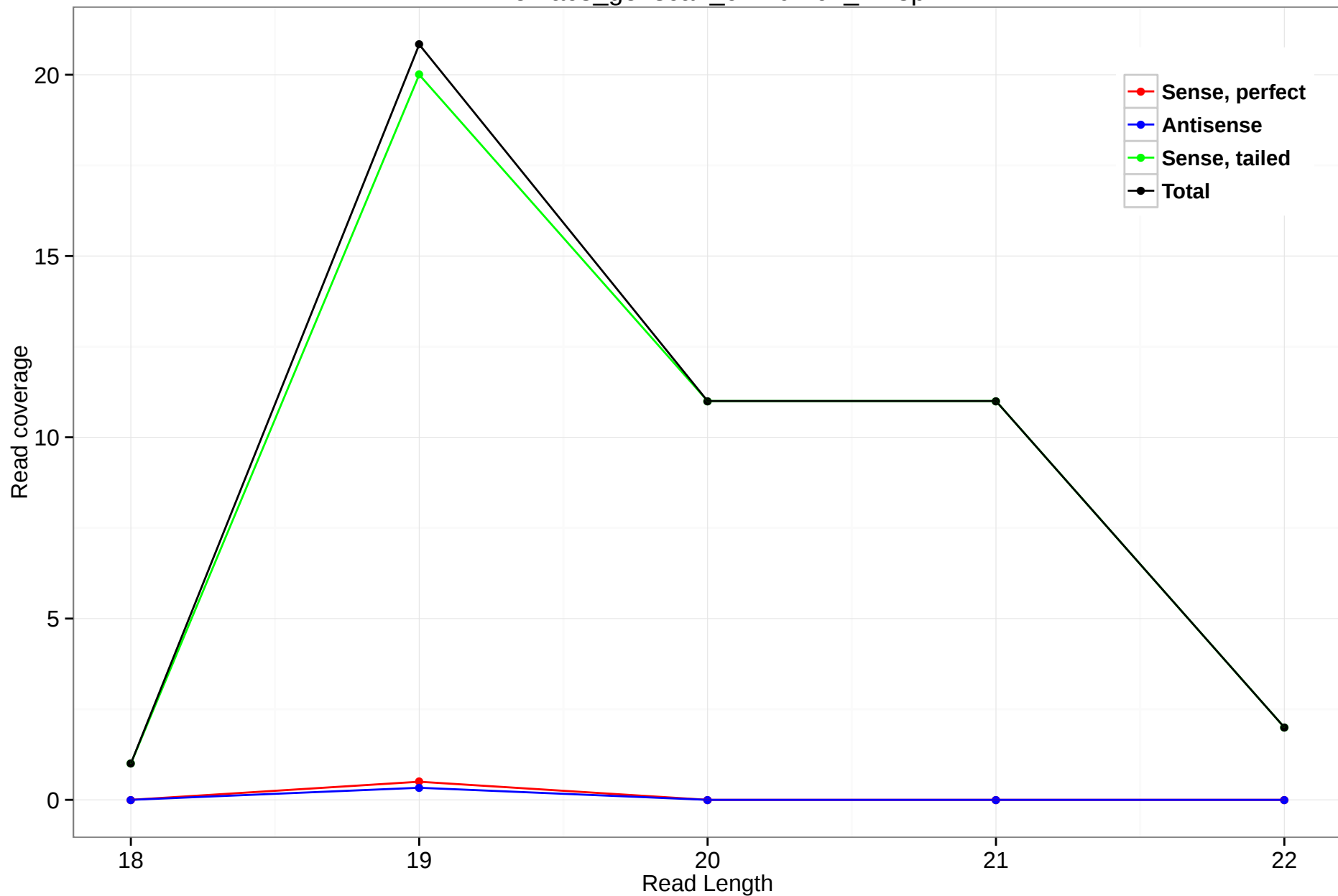
rheMac3_genscan_chr10.762_11.3p
