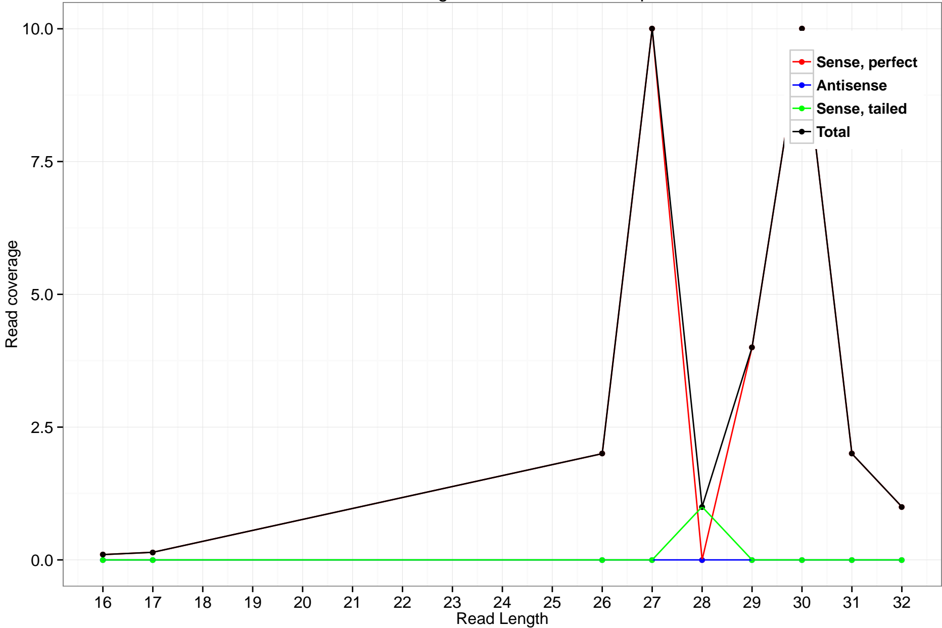
rheMac3_genscan_chr10.740_4.5p
