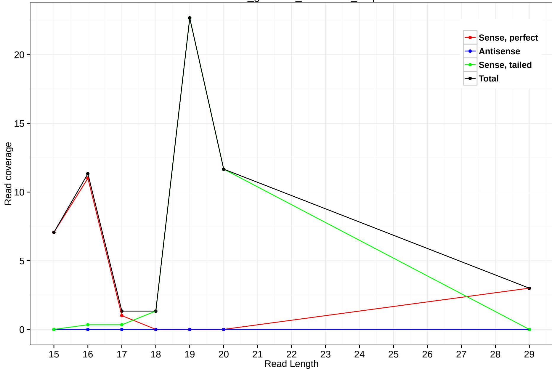
rheMac3_genscan_chr10.697_2.5p
