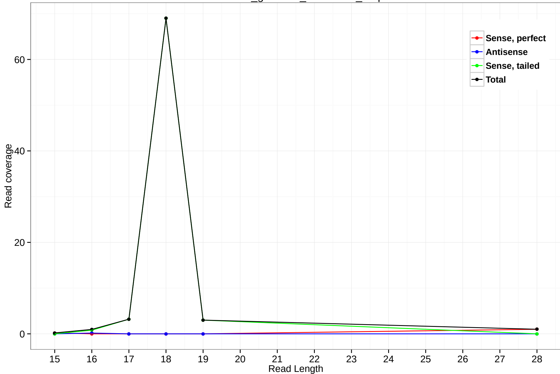
rheMac3_genscan_chr10.691_6.5p
