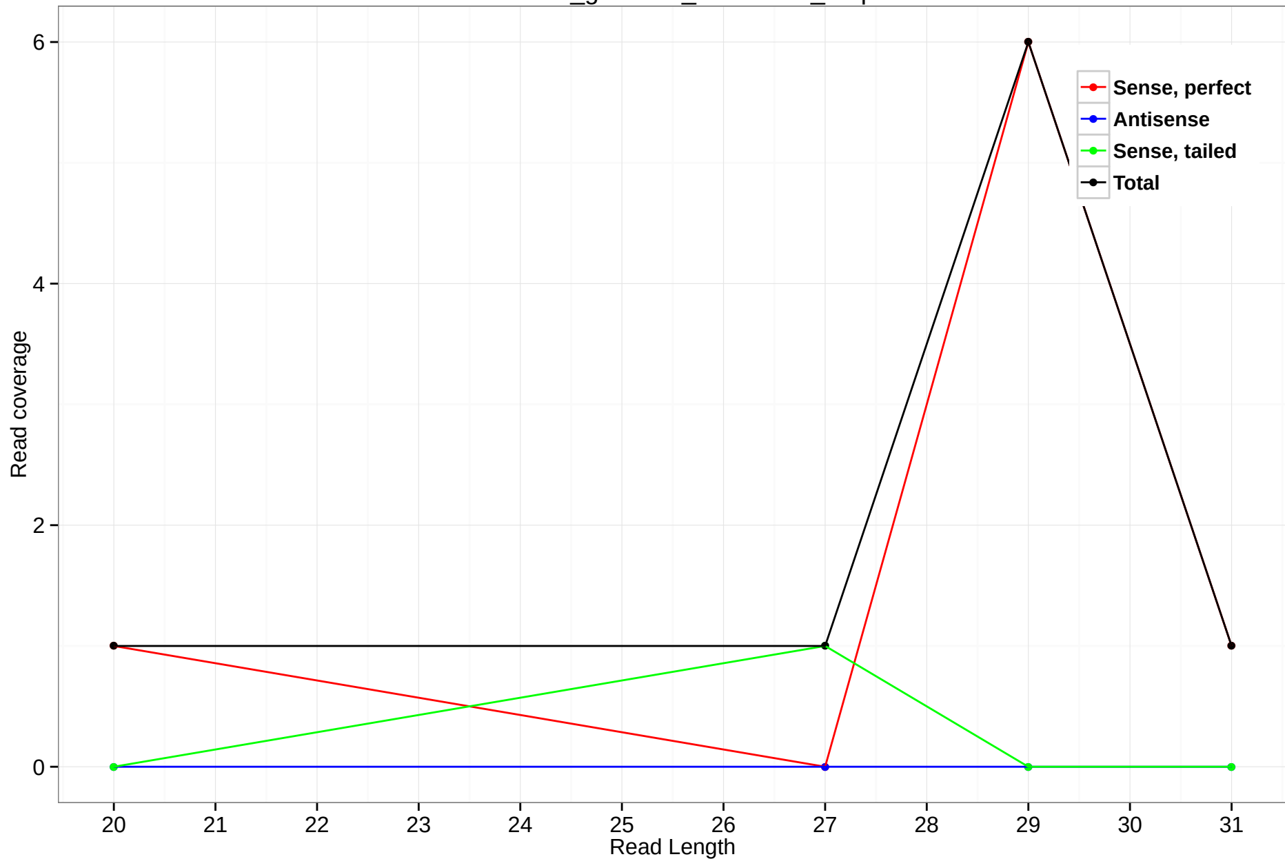
rheMac3_genscan_chr10.688_8.3p
