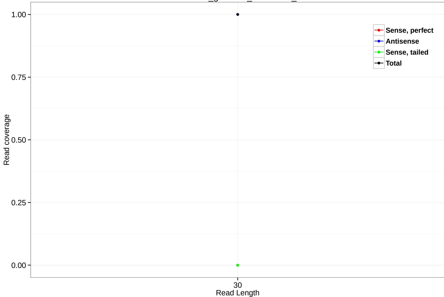
rheMac3_genscan_chr10.684_4
