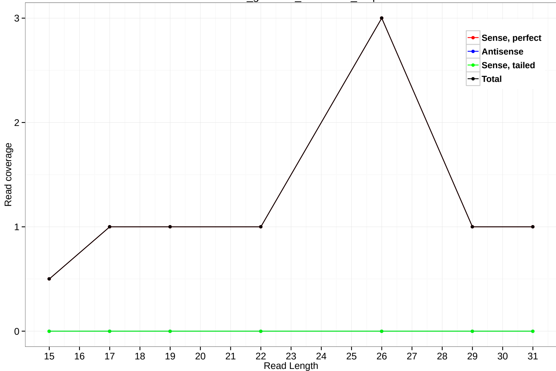
rheMac3_genscan_chr10.682_9.5p
