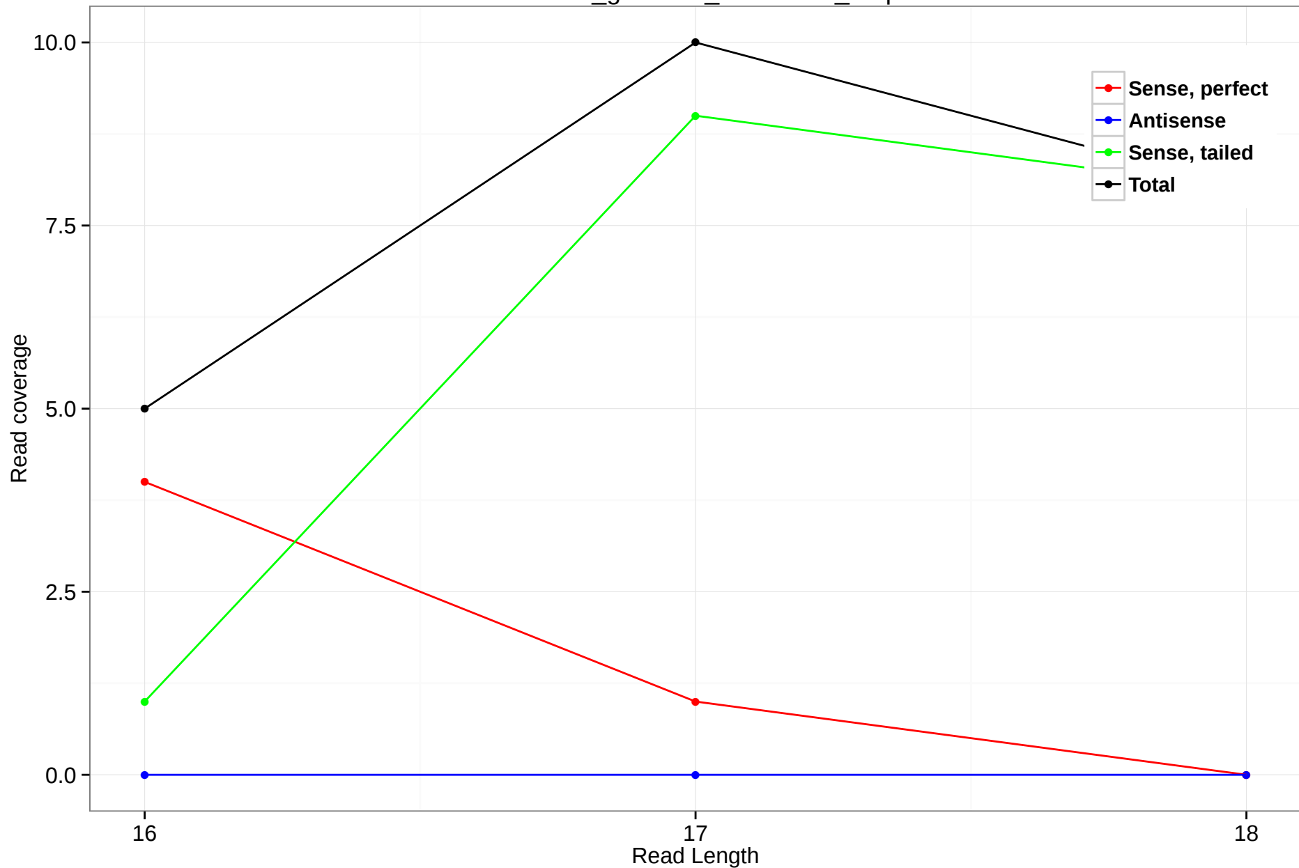
rheMac3_genscan_chr10.682_2.3p
