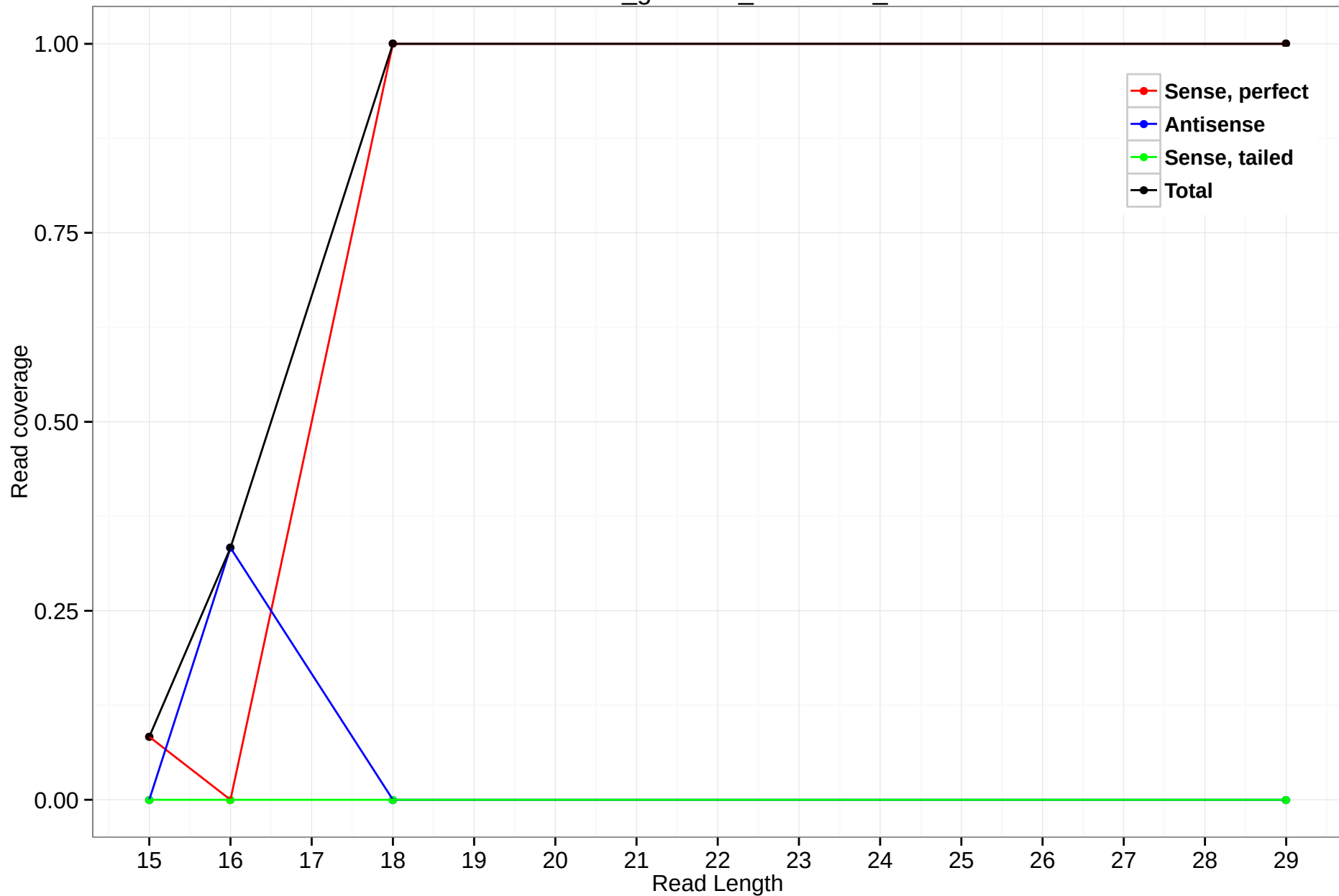
rheMac3_genscan_chr10.662_16
