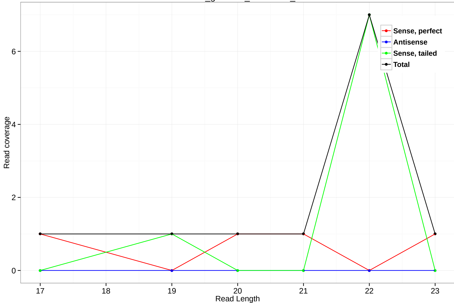
rheMac3_genscan_chr10.662_14
