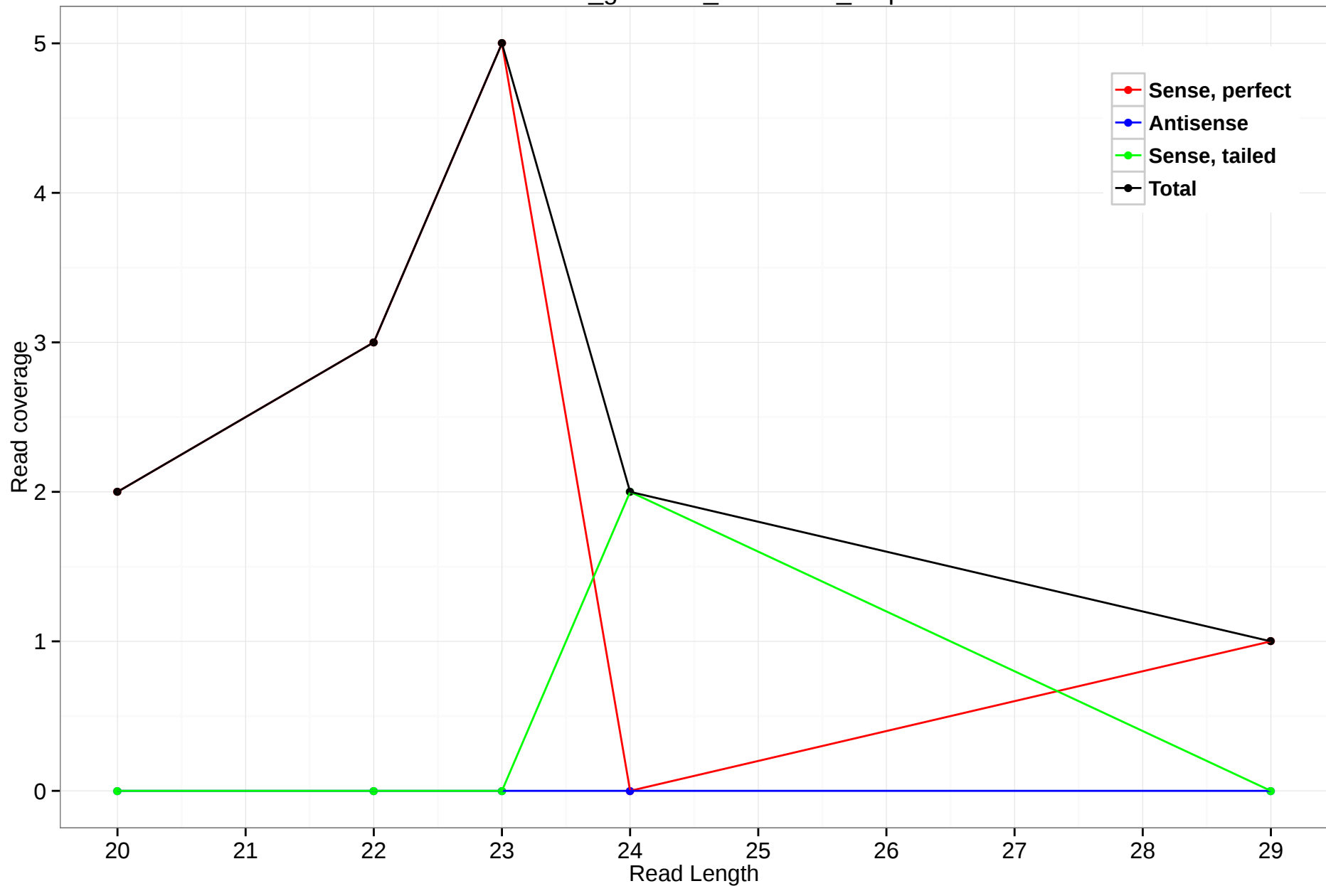
rheMac3_genscan_chr10.629_2.3p
