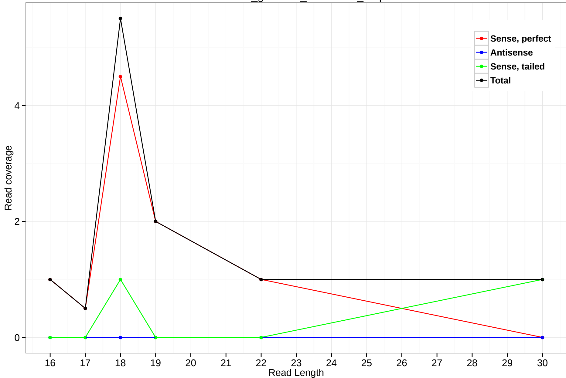
rheMac3_genscan_chr10.625_8.5p
