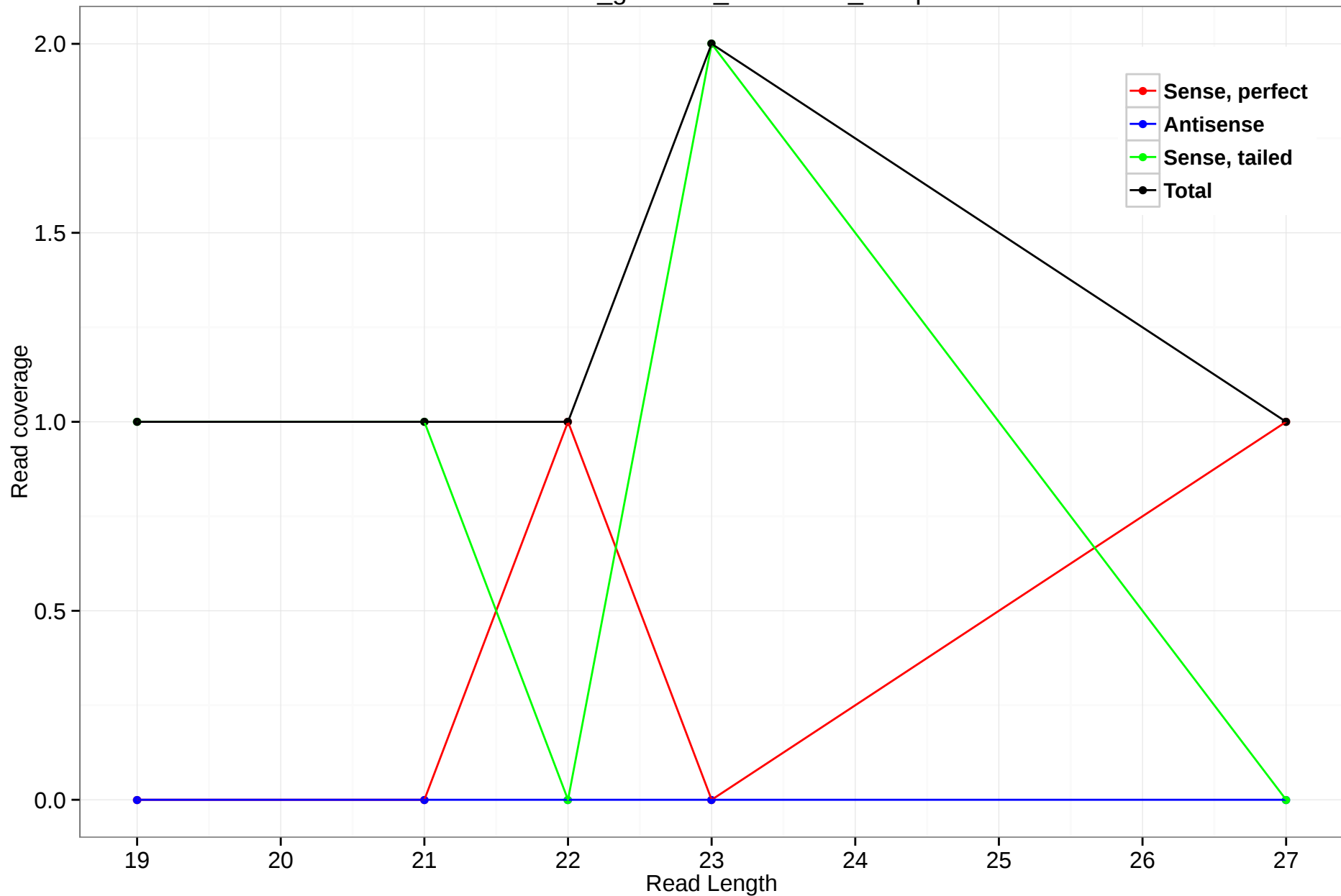
rheMac3_genscan_chr10.617_27.5p
