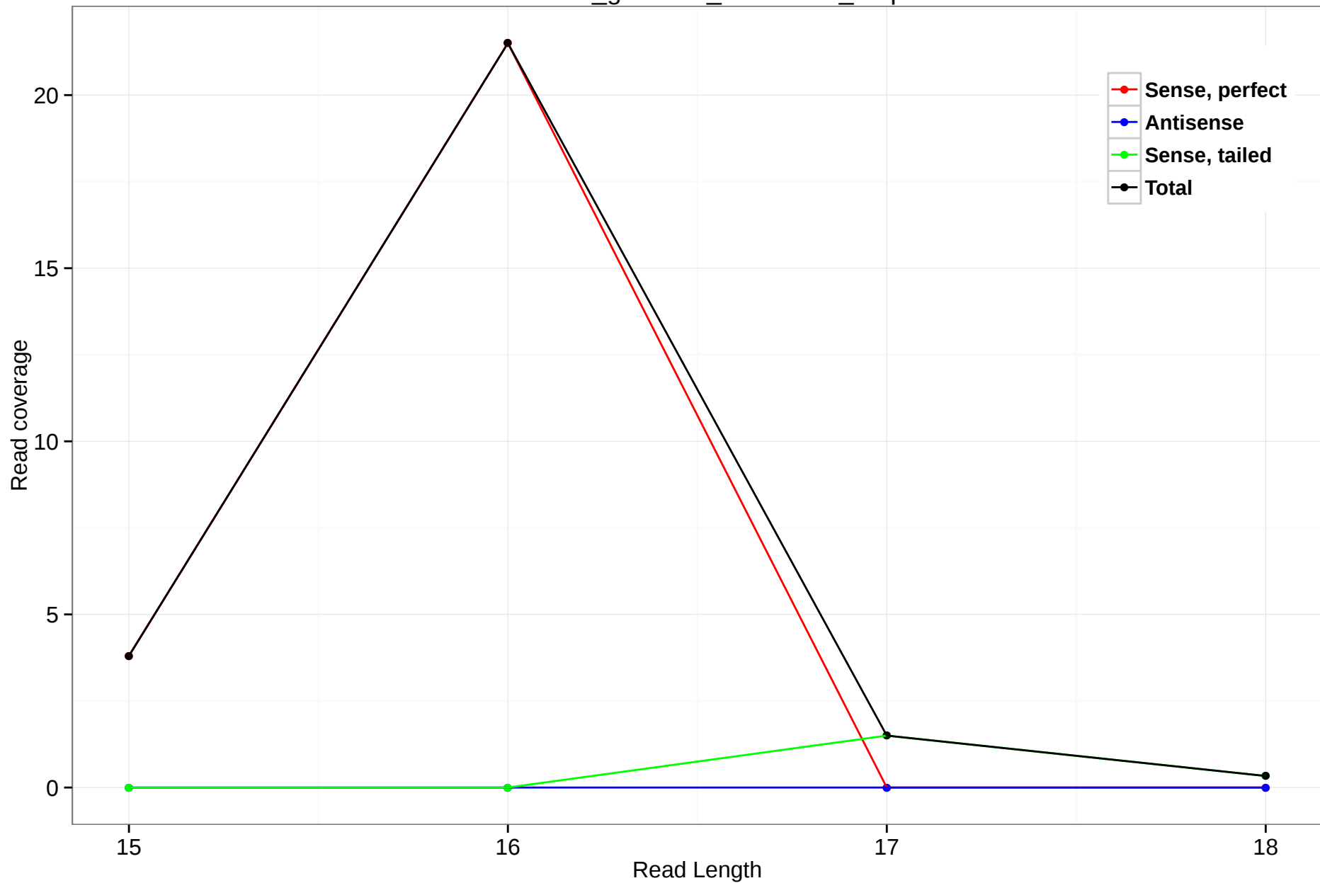
rheMac3_genscan_chr10.594_0.5p
