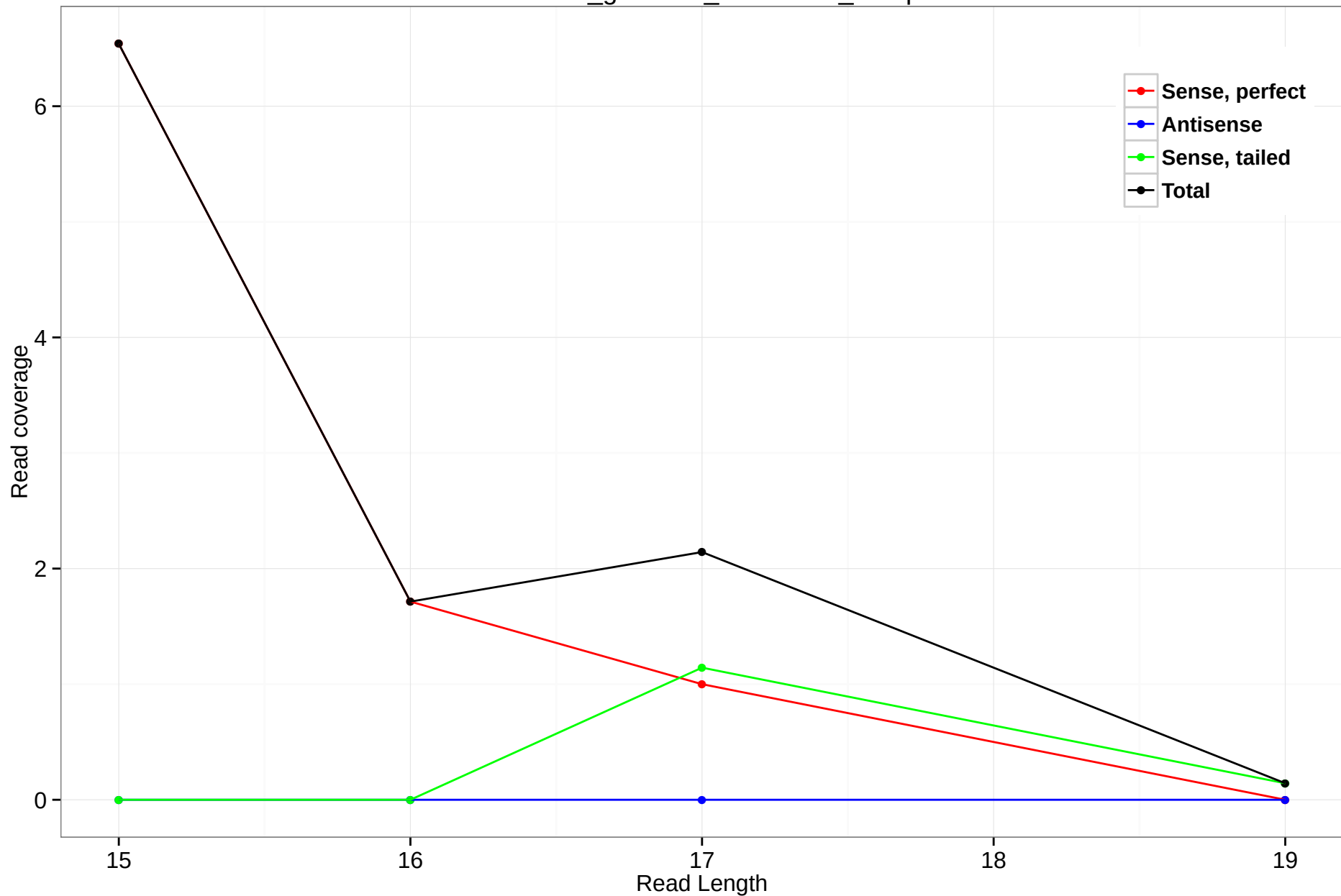
rheMac3_genscan_chr10.523_13.3p
