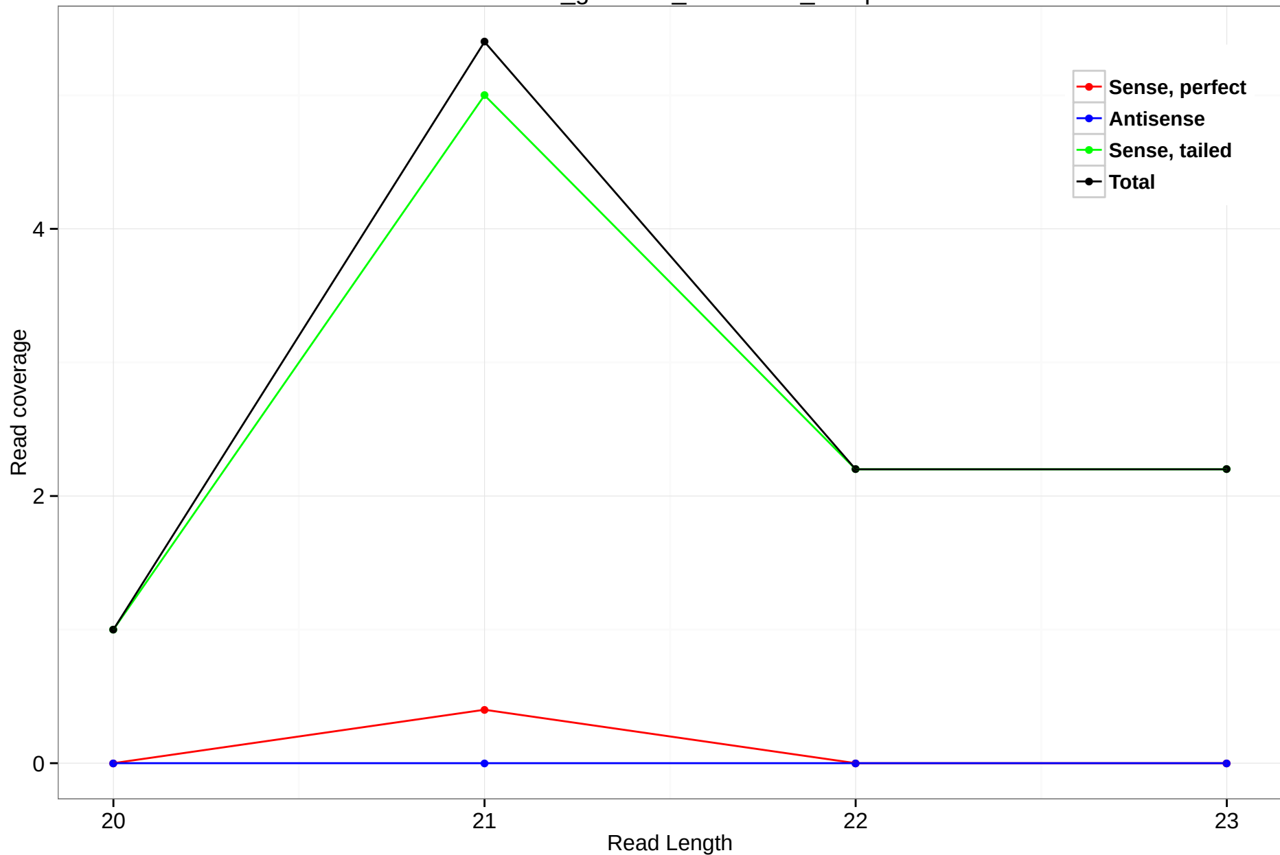
rheMac3_genscan_chr10.521_15.3p
