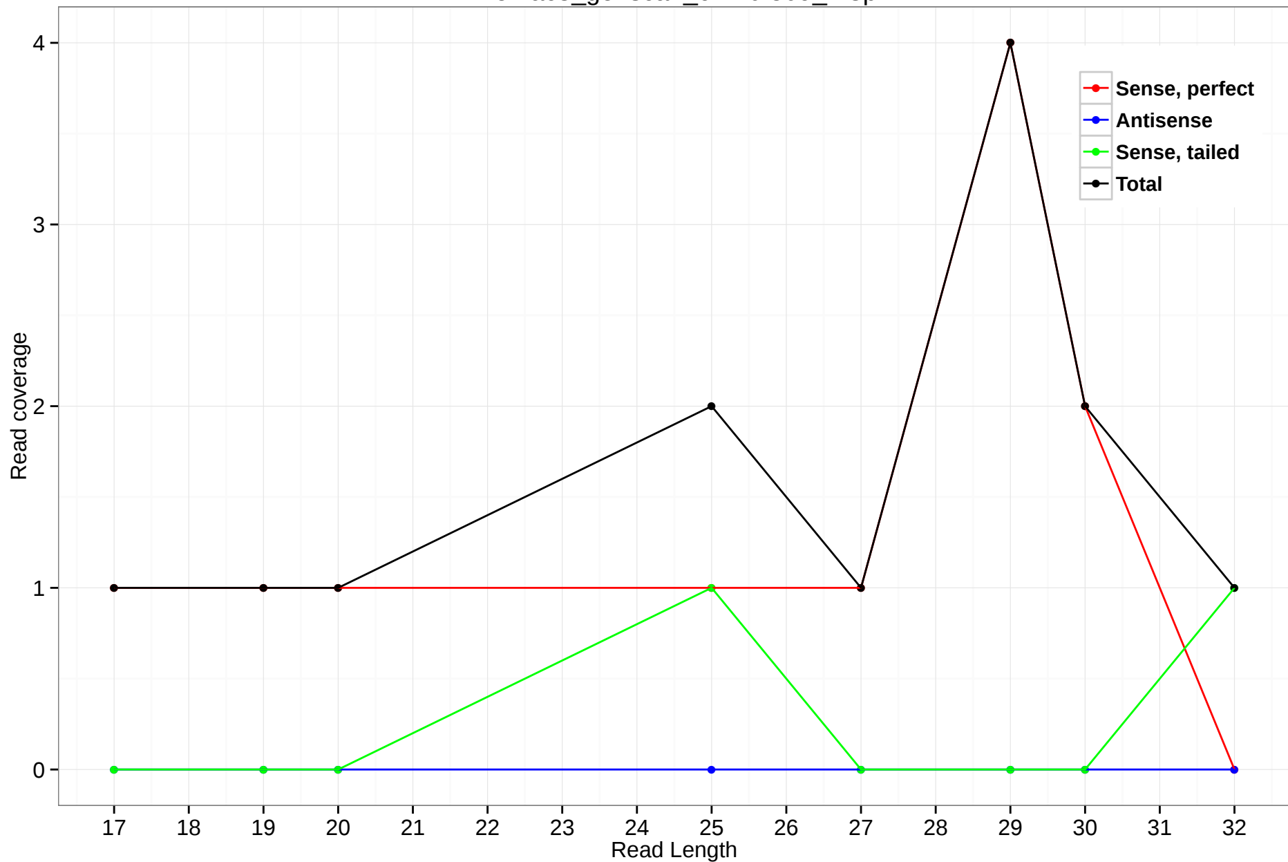
rheMac3_genscan_chr10.509_2.3p
