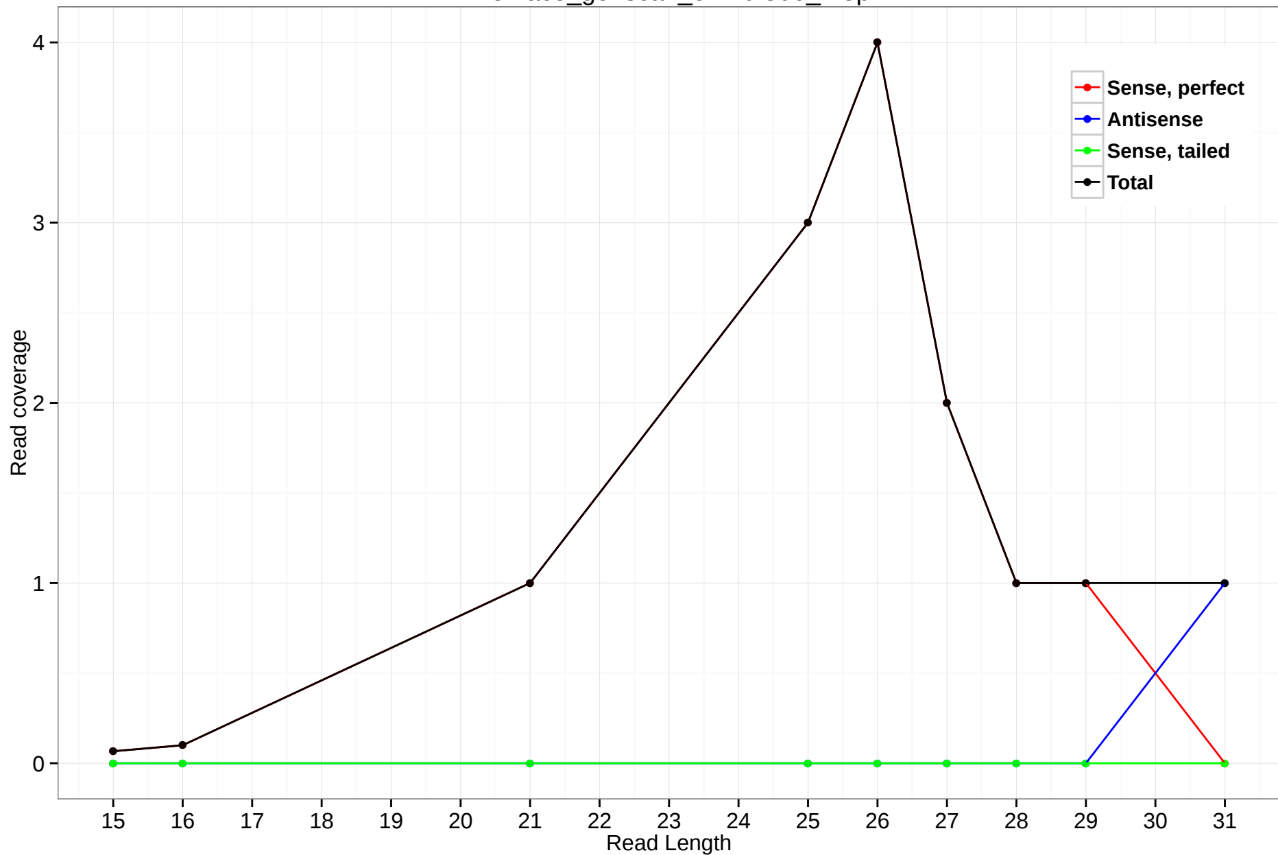
rheMac3_genscan_chr10.506_4.3p
