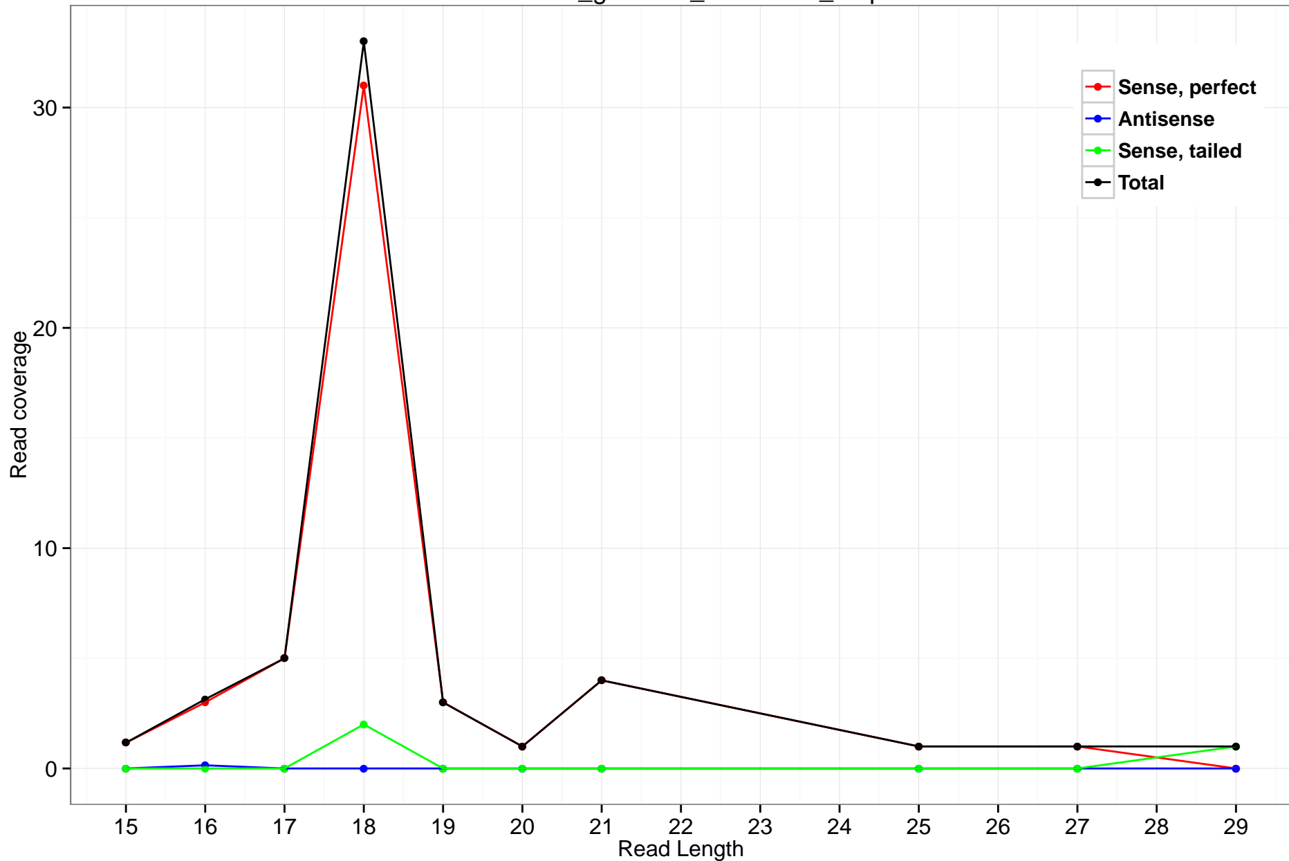
rheMac3_genscan_chr10.462_2.5p
