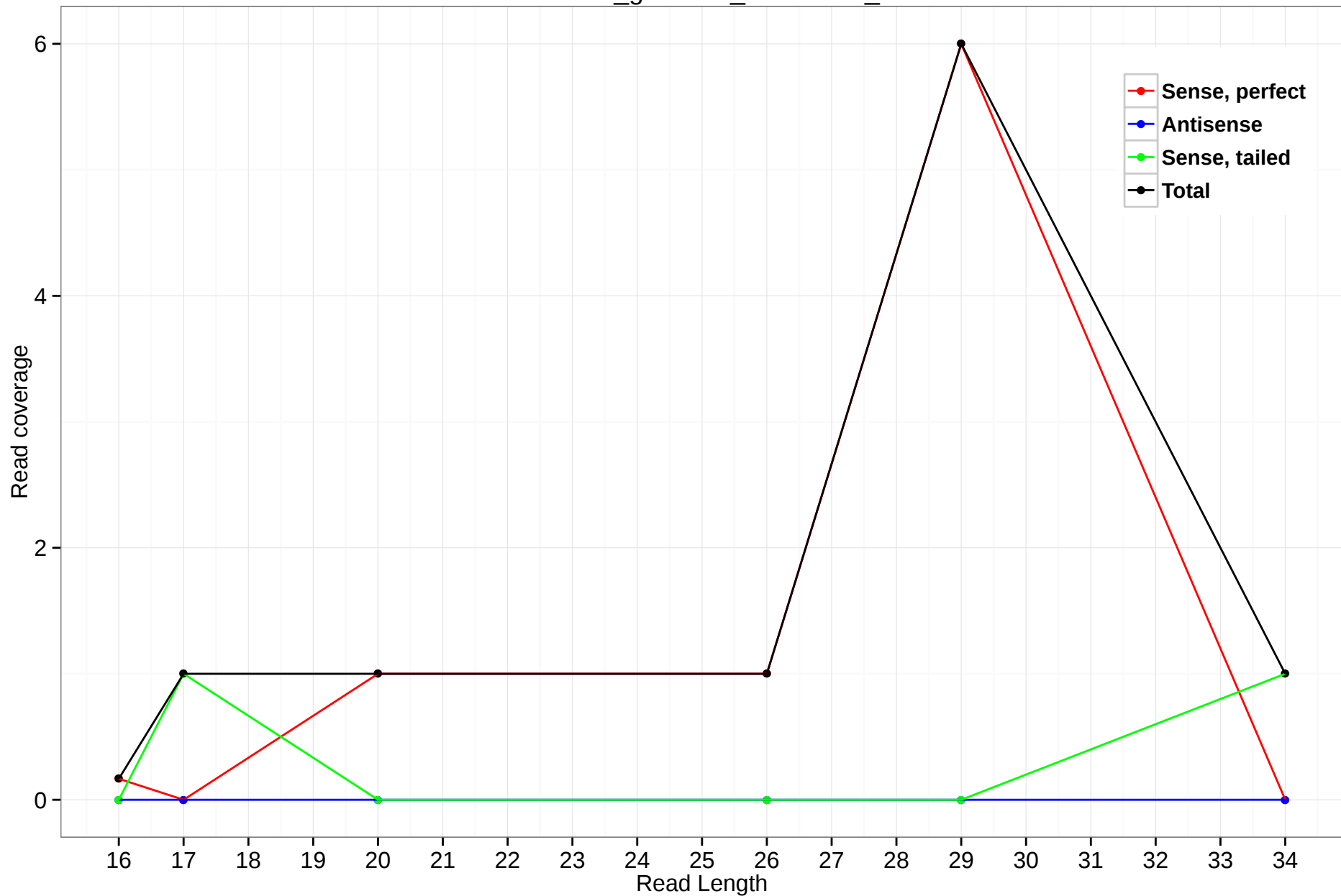
rheMac3_genscan_chr10.459_2
