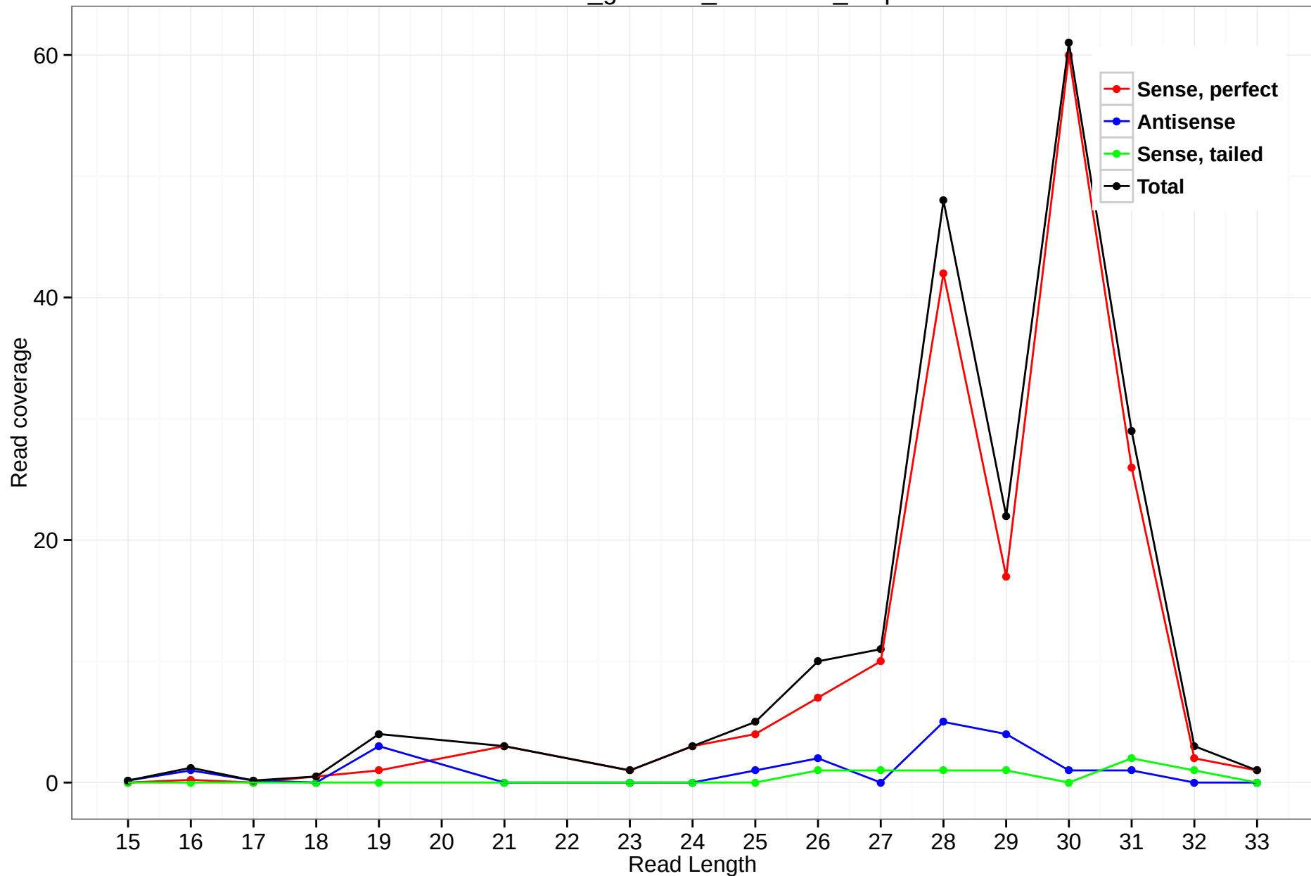
rheMac3_genscan_chr10.378_7.5p
