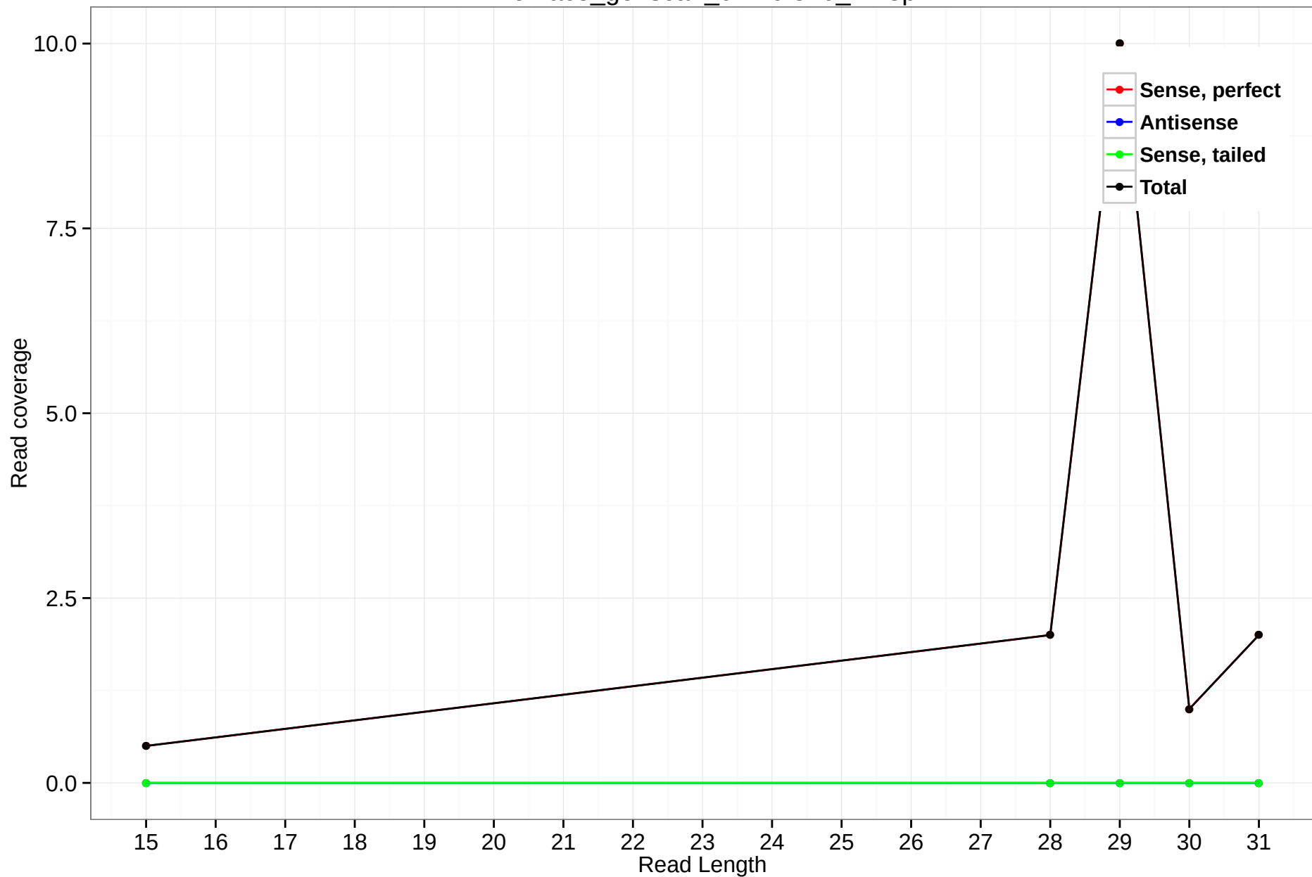
rheMac3_genscan_chr10.370_11.3p
