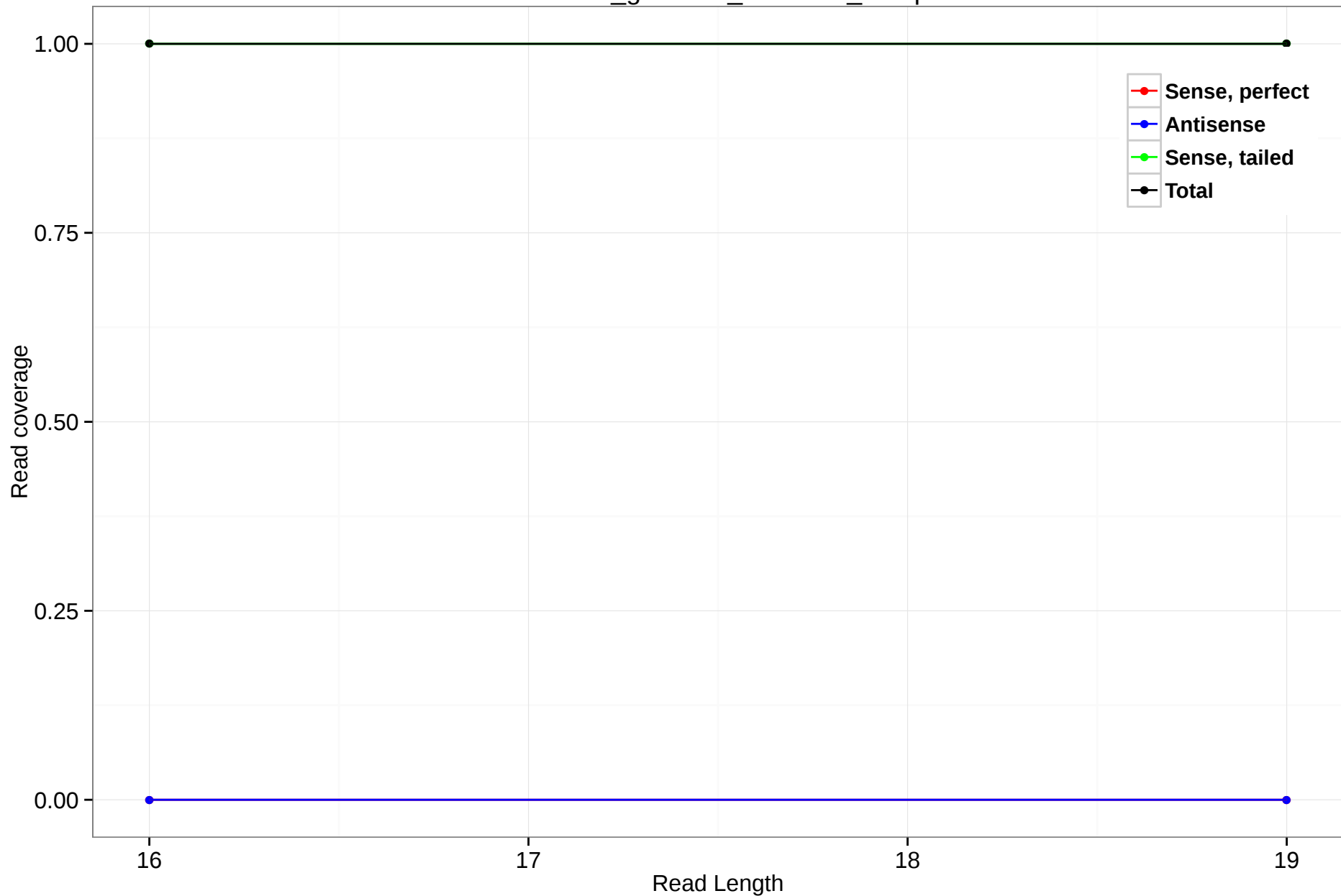
rheMac3_genscan_chr10.34_24.5p
