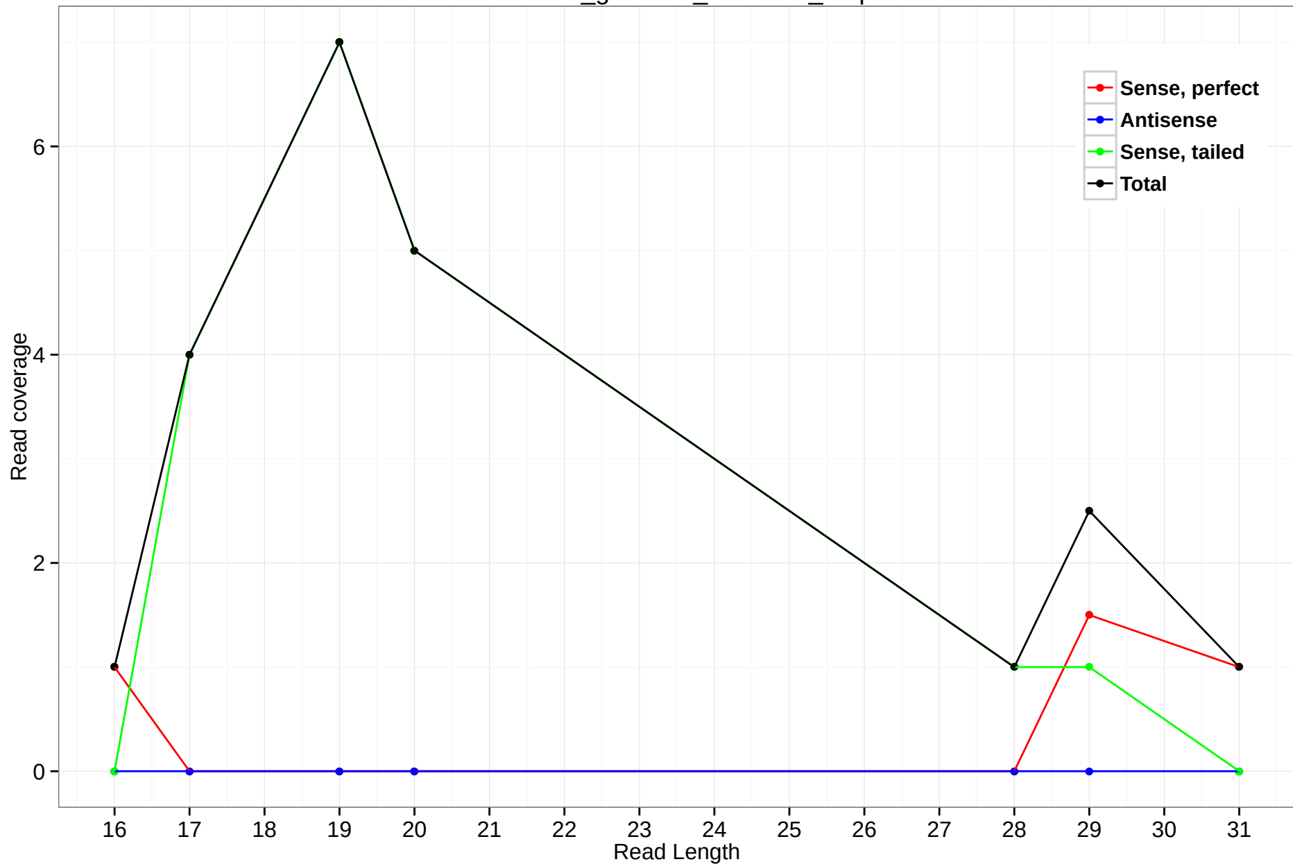
rheMac3_genscan_chr10.25_5.5p
