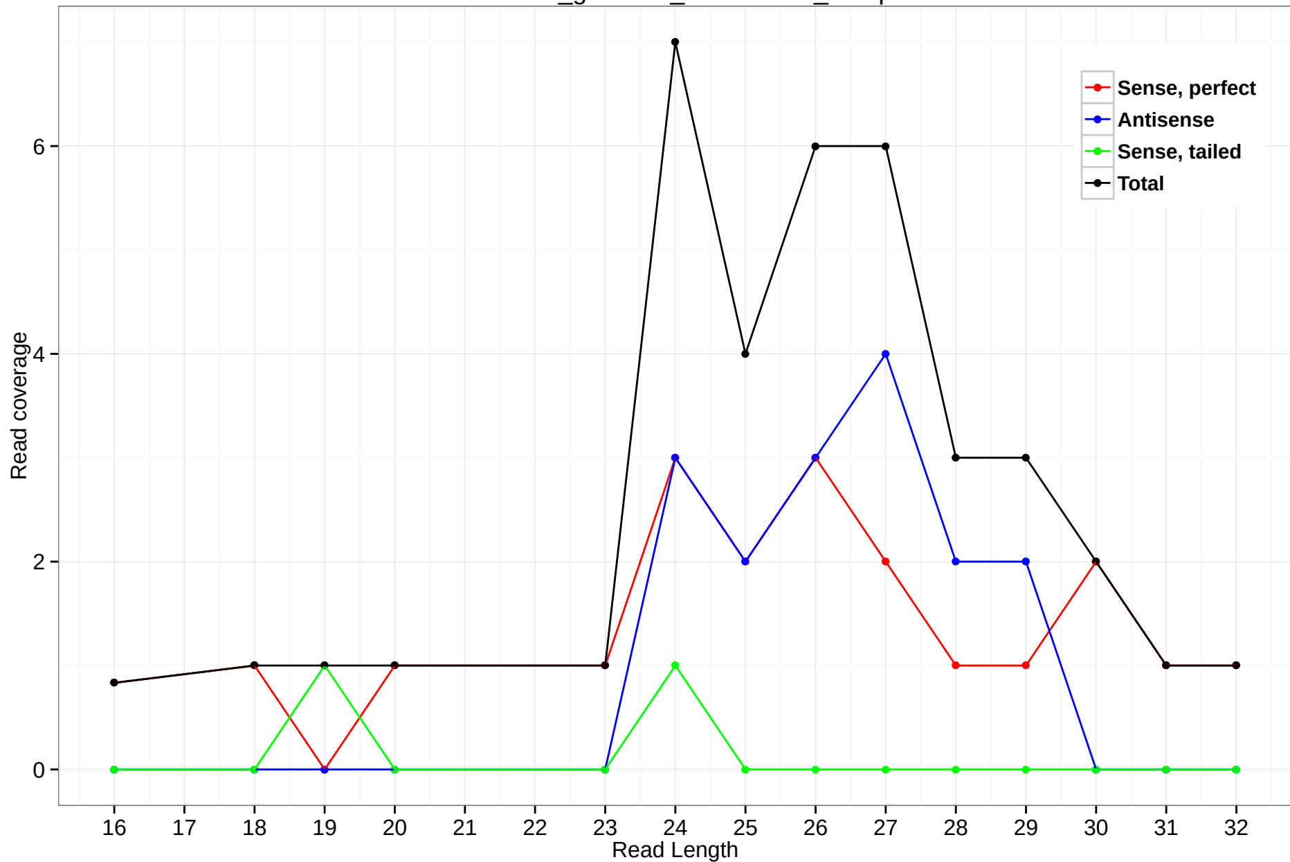
rheMac3_genscan_chr10.2314_26.5p
