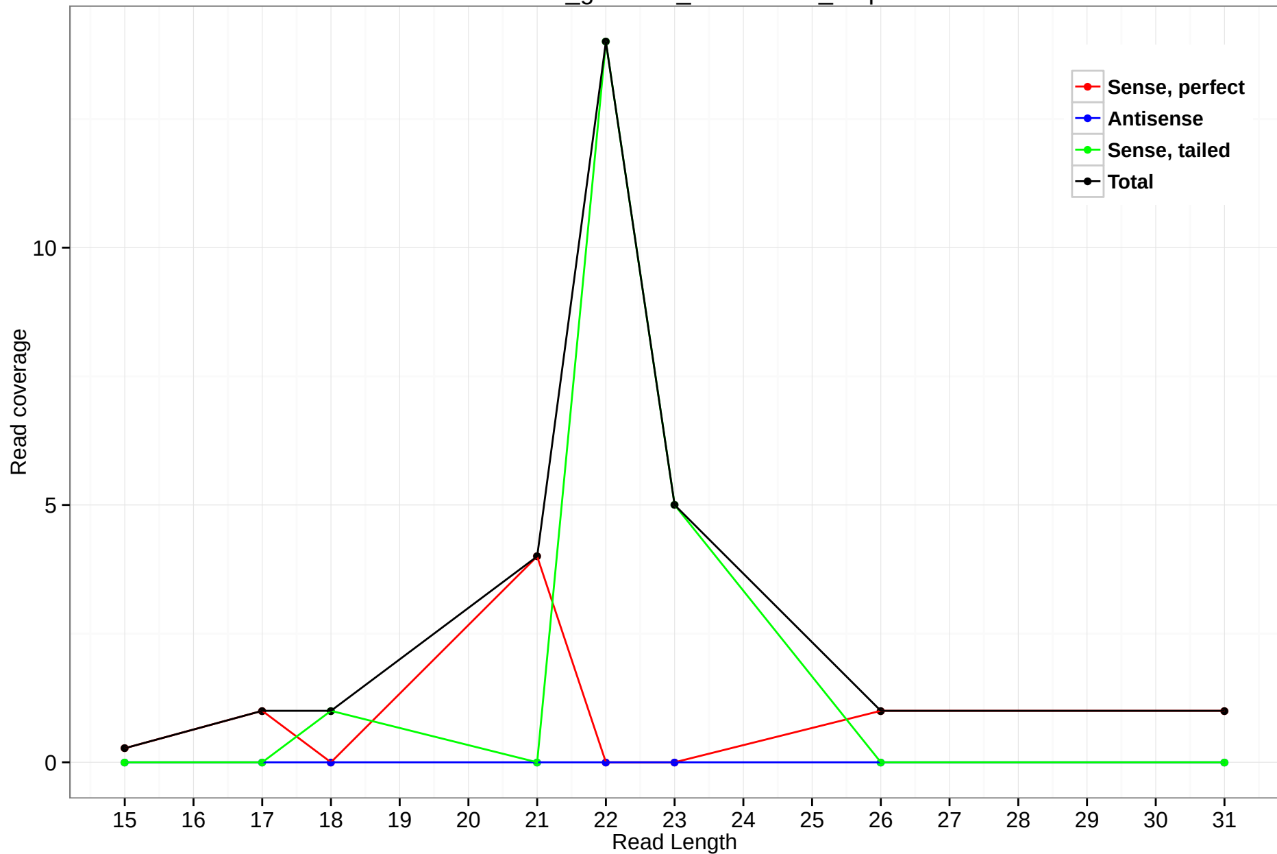
rheMac3_genscan_chr10.2305_8.5p
