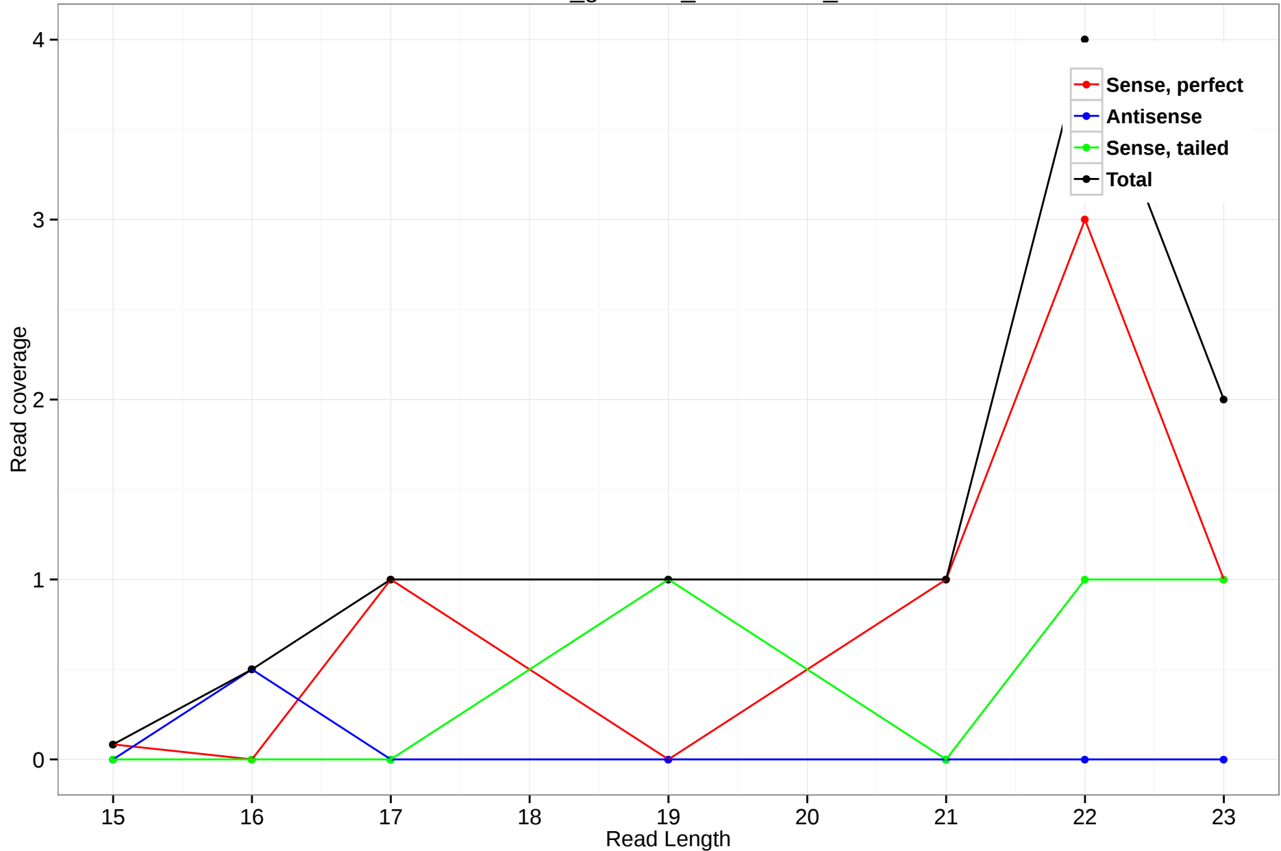
rheMac3_genscan_chr10.2301_39
