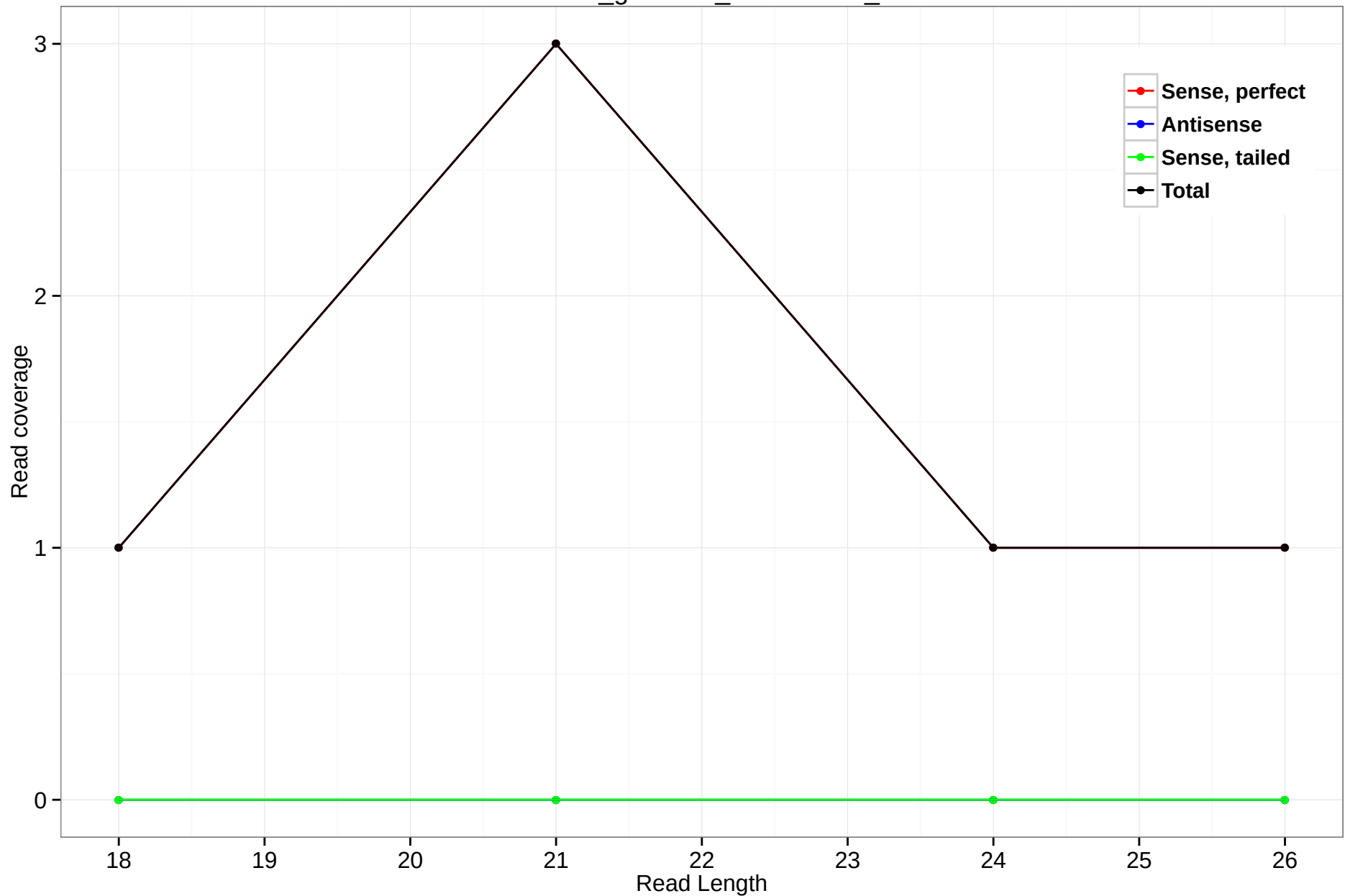
rheMac3_genscan_chr10.2301_37
