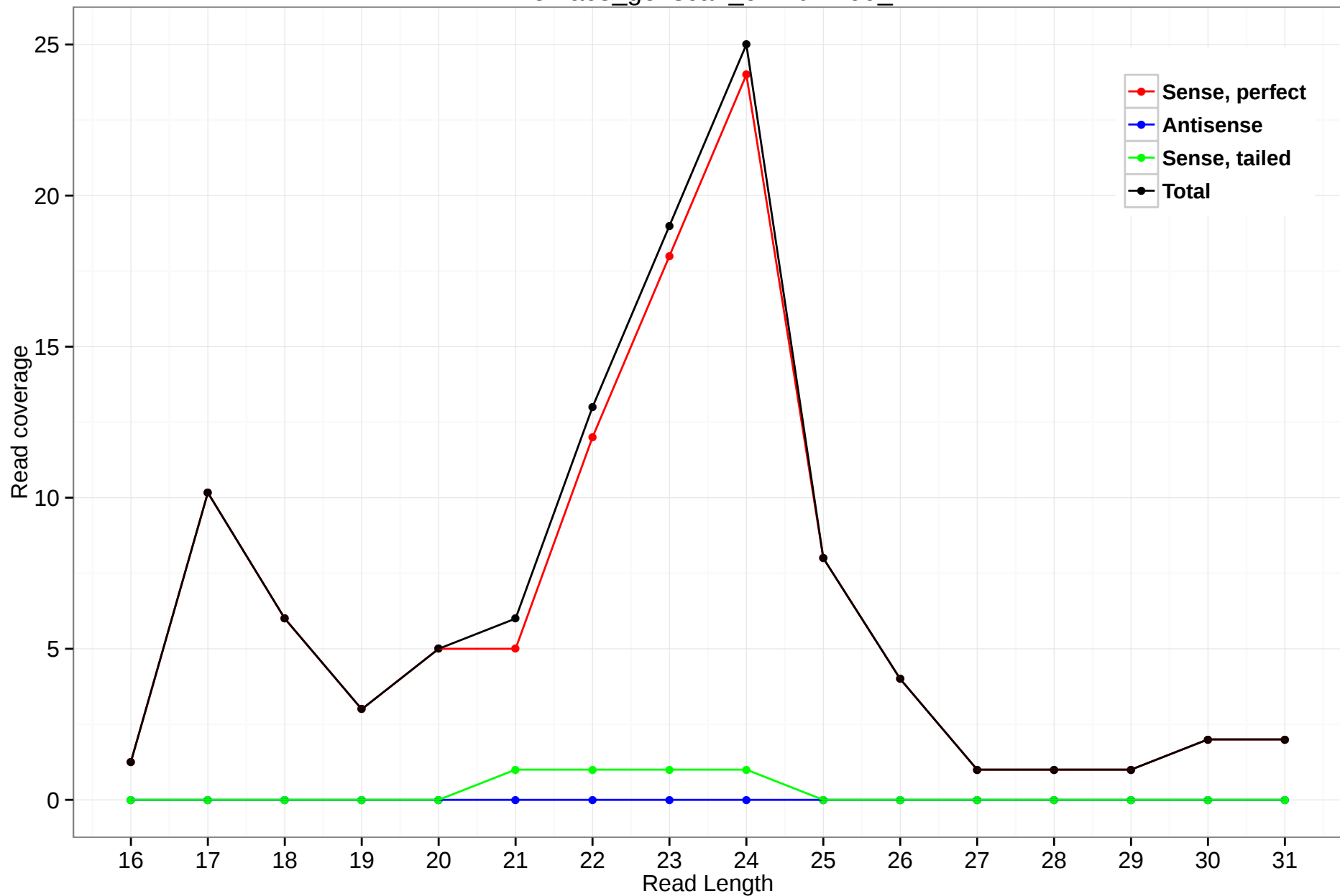
rheMac3_genscan_chr10.2299_7
