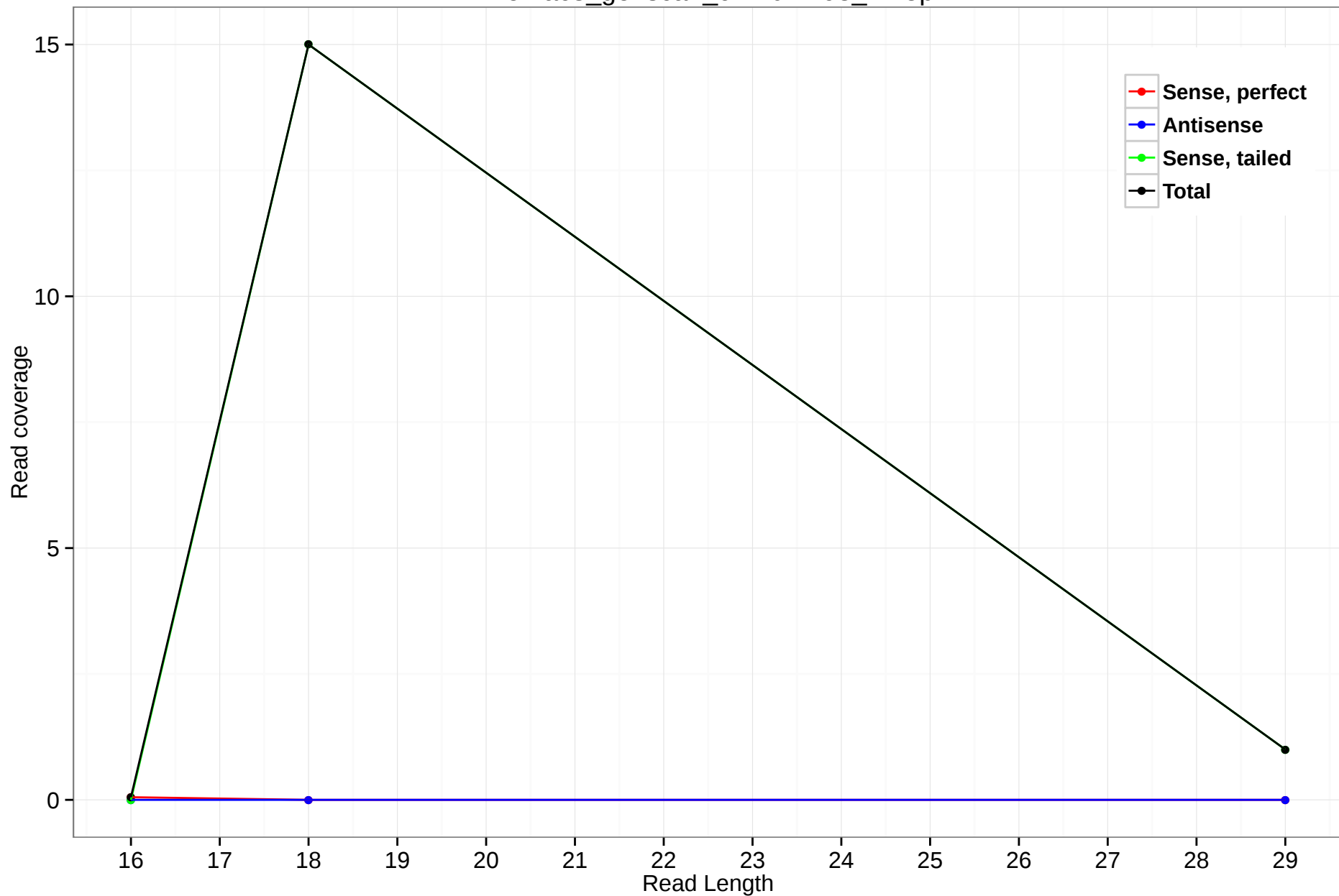
rheMac3_genscan_chr10.2298_44.5p
