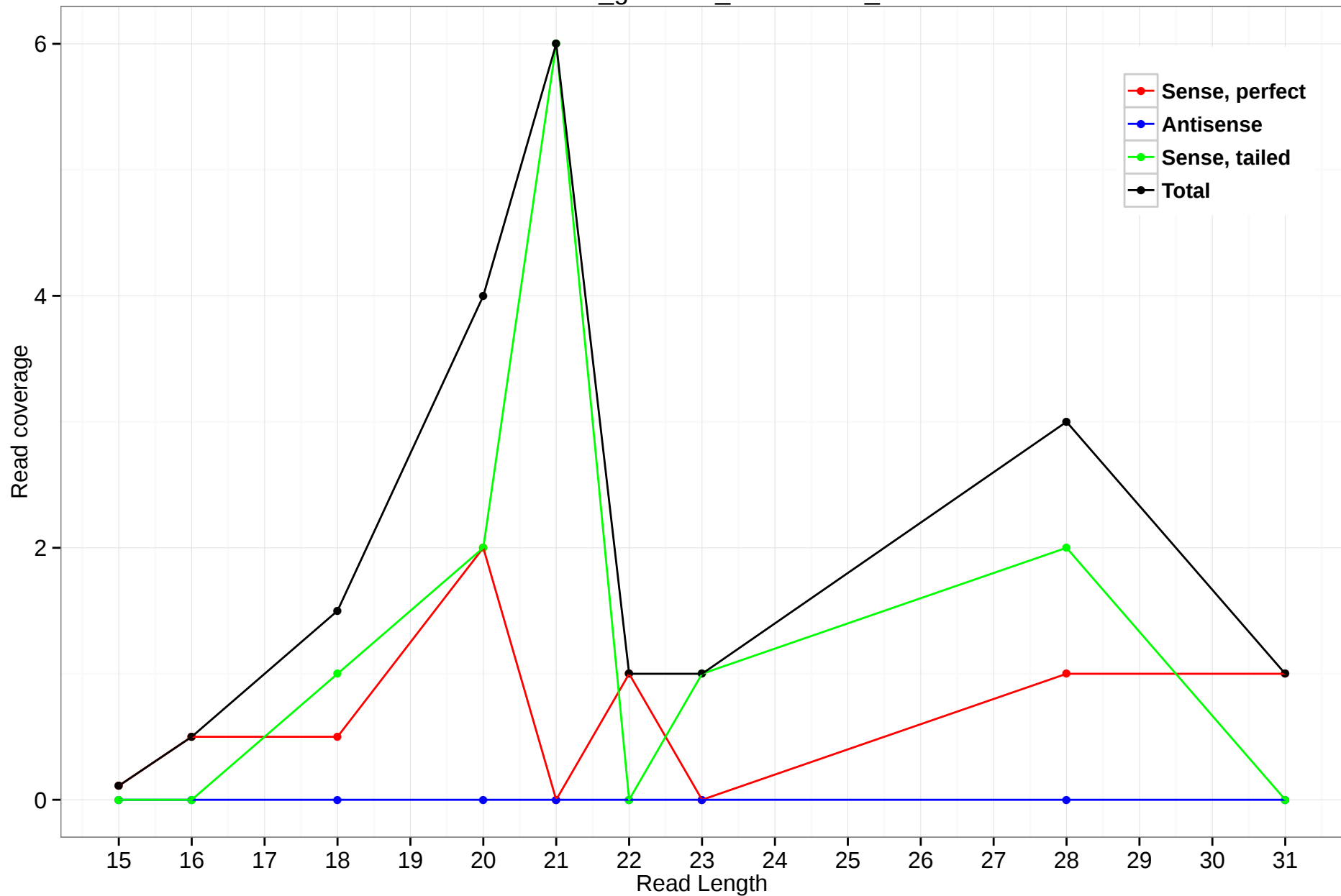
rheMac3_genscan_chr10.2298_33
