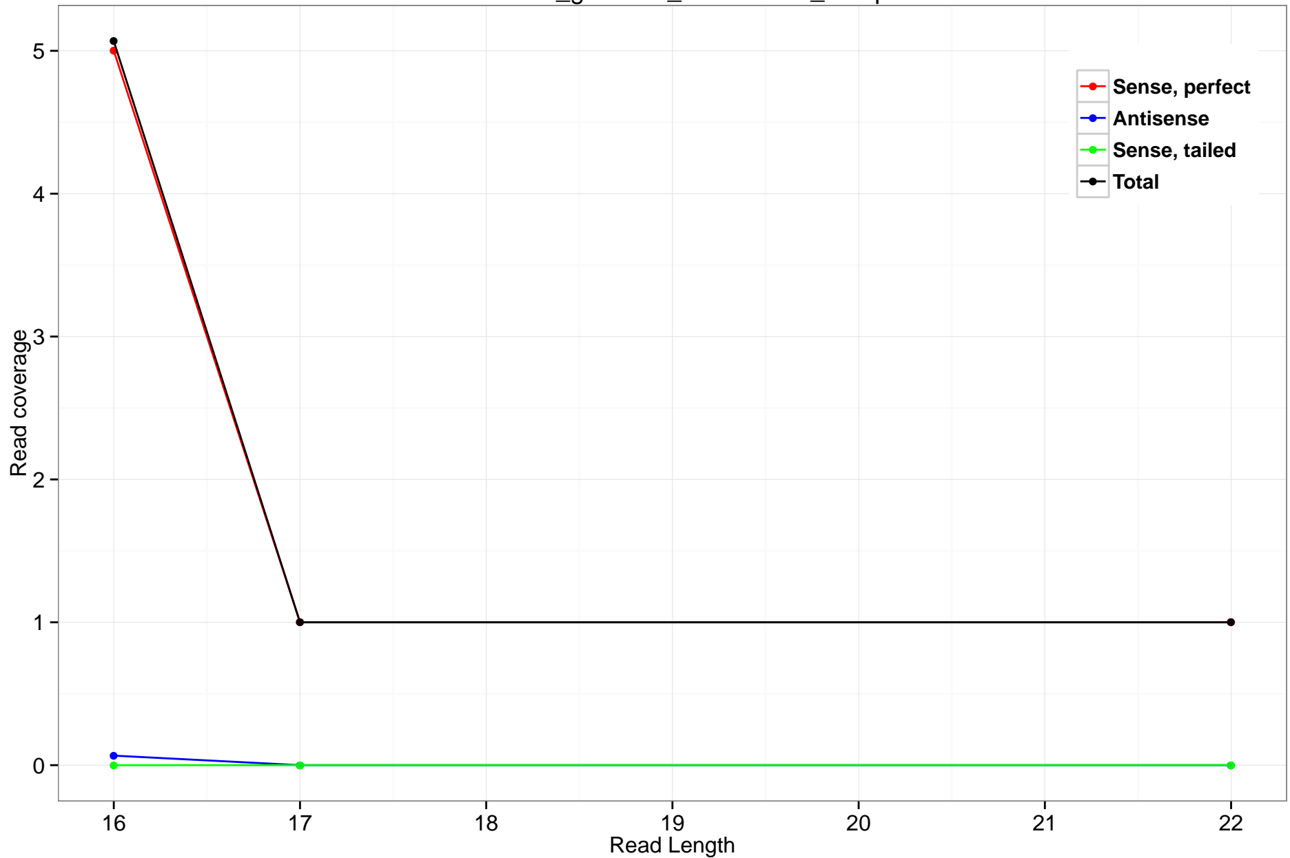
rheMac3_genscan_chr10.2298_31.5p
