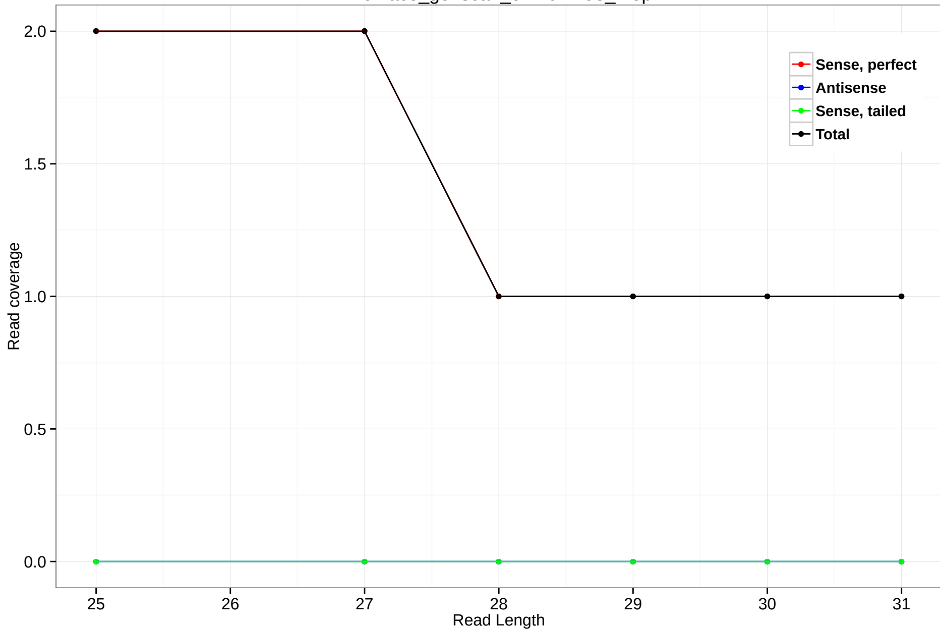
rheMac3_genscan_chr10.2293_1.5p
