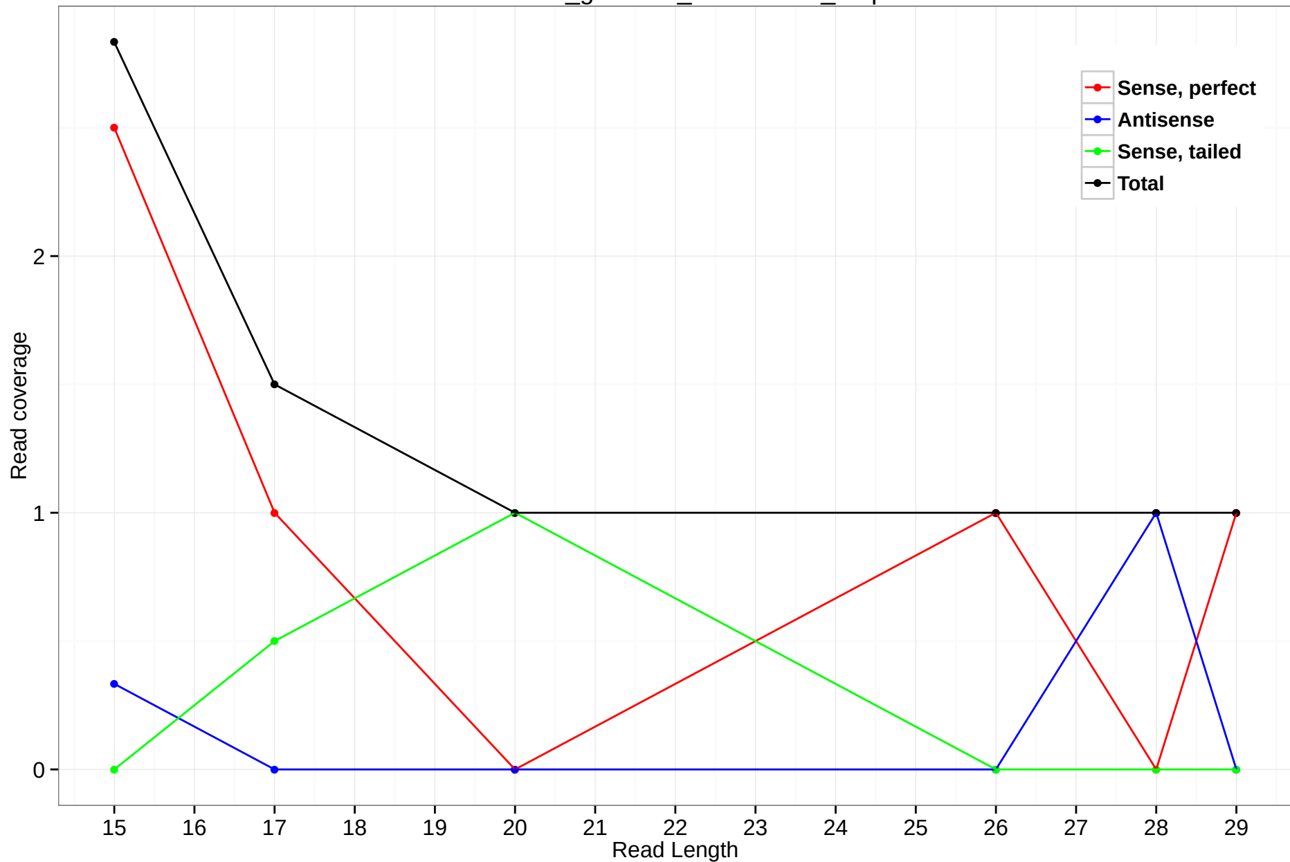
rheMac3_genscan_chr10.2270_6.5p
