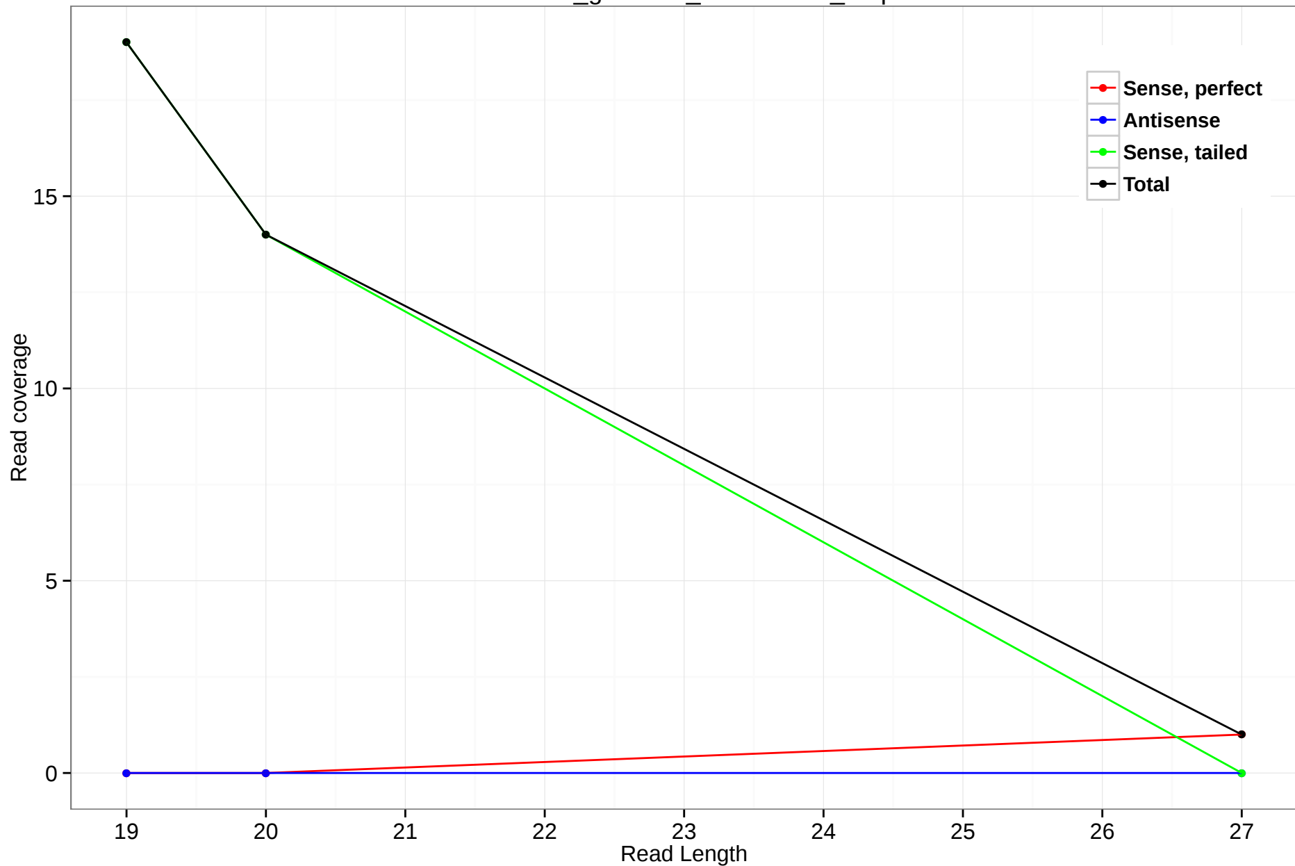
rheMac3_genscan_chr10.2170_1.3p
