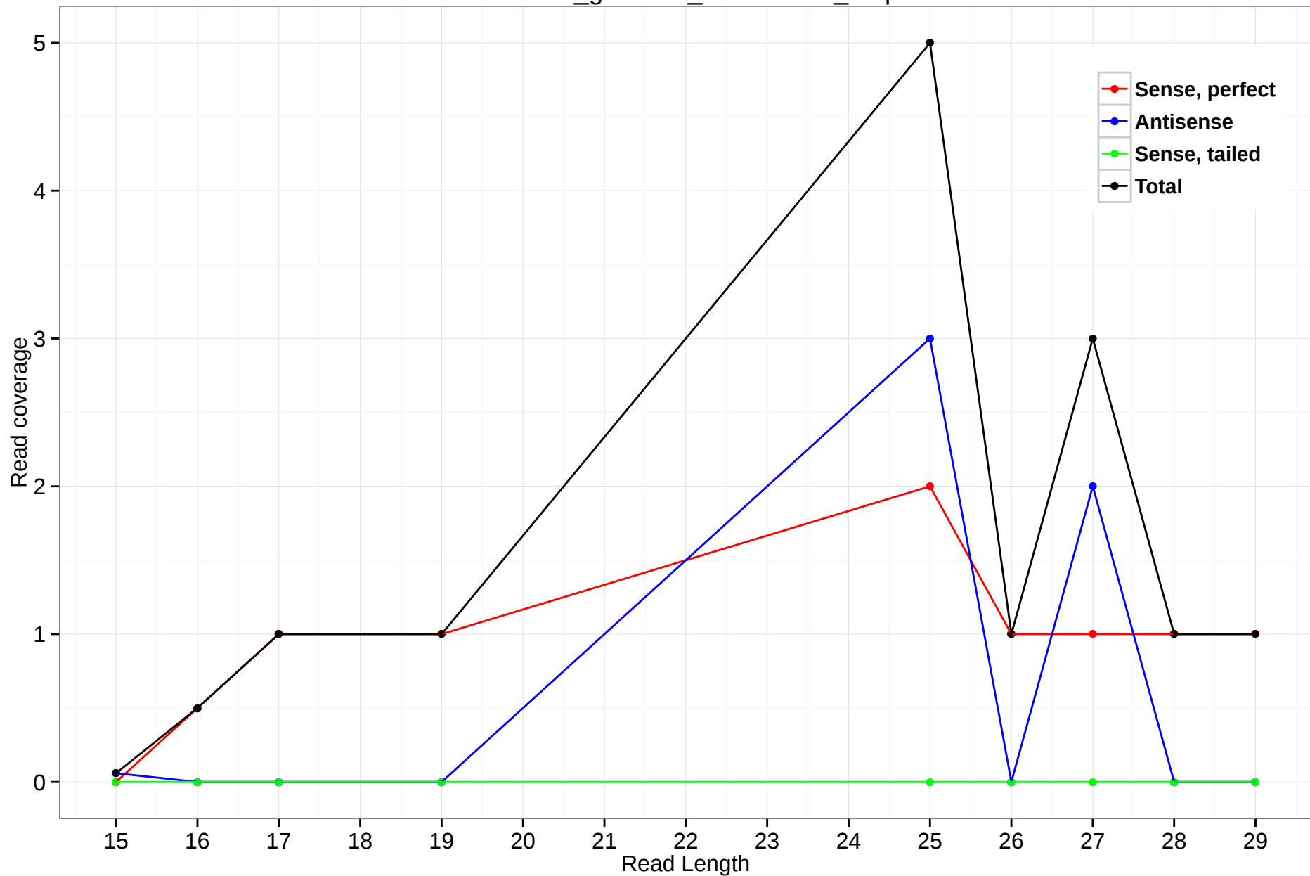
rheMac3_genscan_chr10.2118_3.3p
