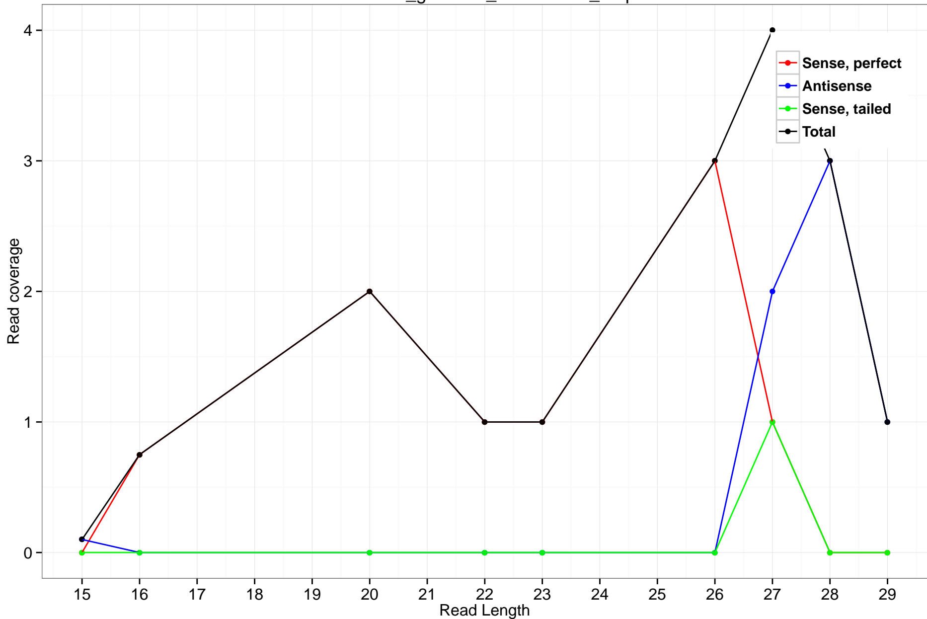
rheMac3_genscan_chr10.2118_2.5p
