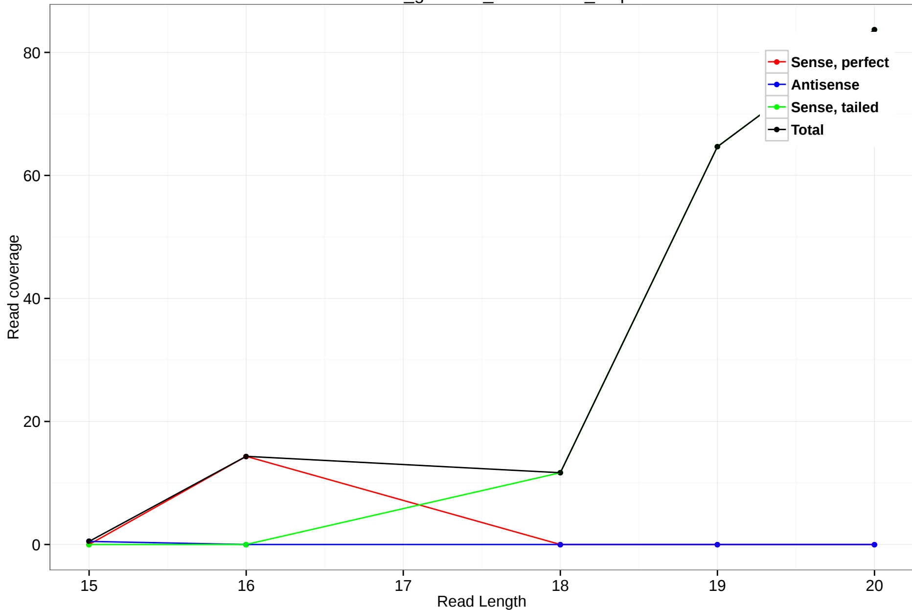
rheMac3_genscan_chr10.2104_0.3p
