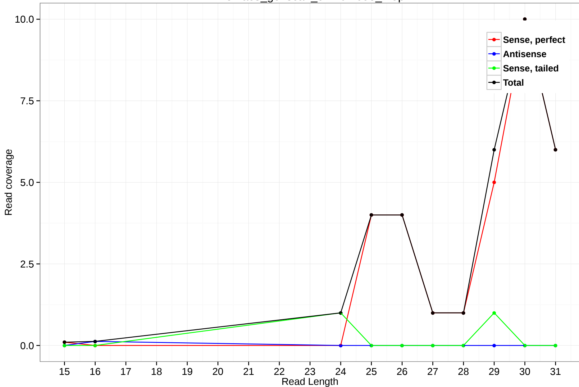
rheMac3_genscan_chr10.2098_2.5p
